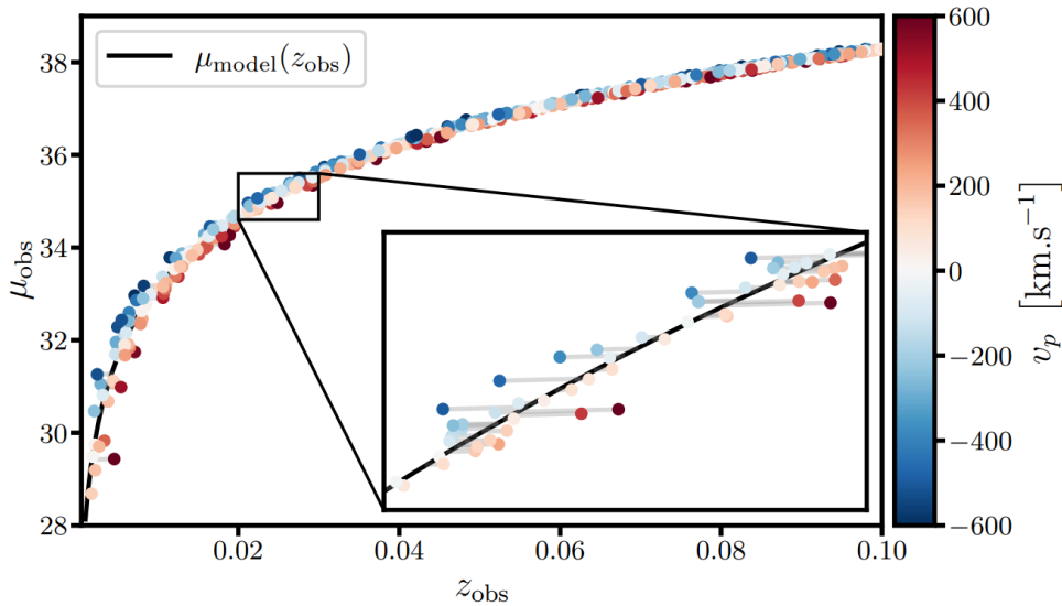
Fig. 2.7 Illustration of the impact of peculiar velocities on the distance modulus on a Hubble diagram from [Carreres et al., 2023]. The velocities were drawn randomly from a Gaussian distribution. The blue and red colors indicate the radial velocity of the supernova.
