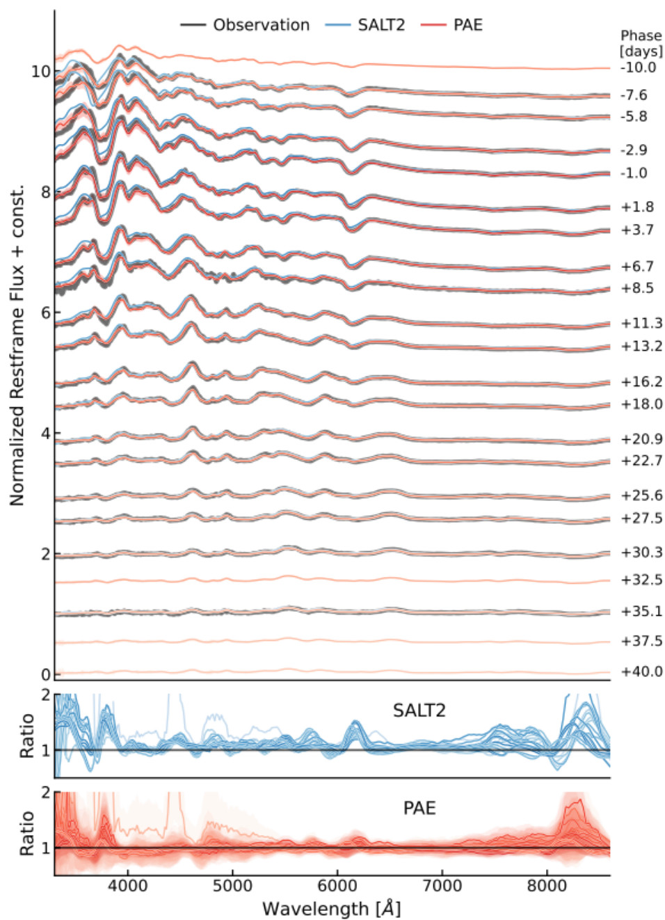
Fig. 2.19 Model comparisons from SuPAErnova (red) and SALT2 (blue) on the spectral series of the SN2010dt supernova observed by SNfactory (black) as well as ratios between model and data. Taken from [Stein et al., 2022]
