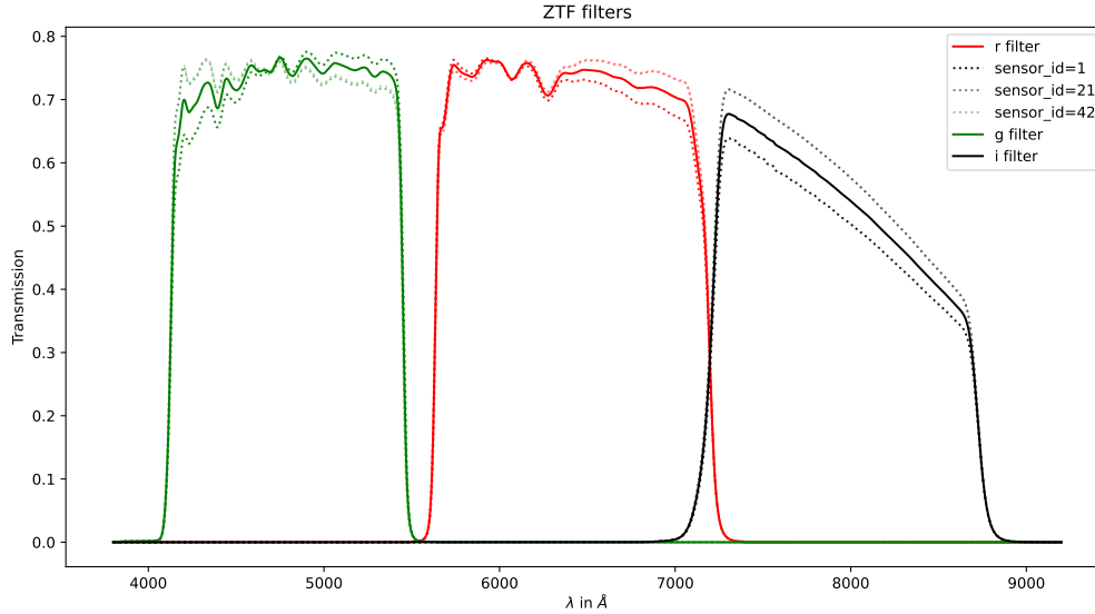
Fig. 3.5 ZTF filters. Dotted lines represent transmissions for different sensors. Solid lines represent the average transmissions over all sensors.
