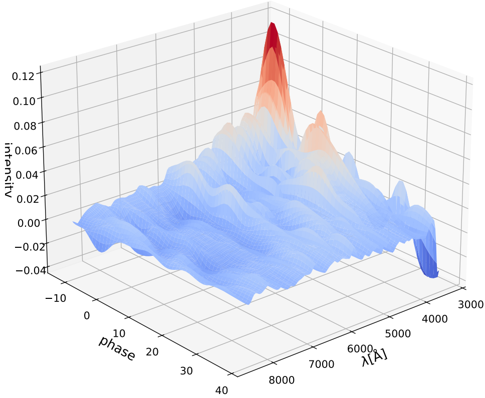
Fig. 2.13 The SALT2.4 M_1 surface with respect to the restframe wavelength and phase
