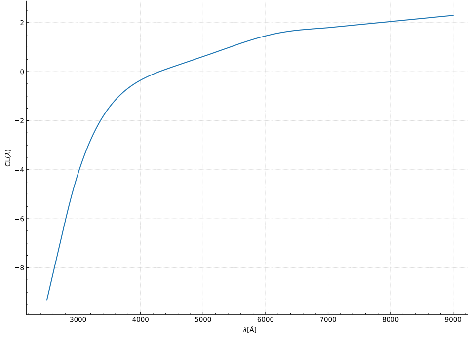
Fig. 2.14 The SALT2.4 color law CL surface with respect to the restframe wavelength
