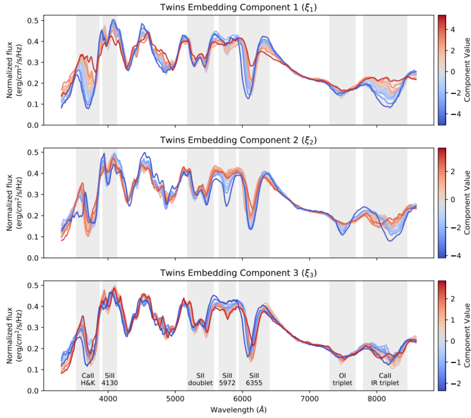
Fig. 2.18 Variations of the Twins Embedding model near maximum light when varying each one of its components \xi_1 , \xi_2 and \xi_3 . For each component, the spectrum shown is the median of 20 evenly populated bins of the coordinates of that component. Taken from [Boone et al., 2021].
