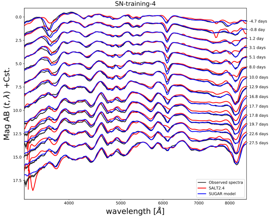
Fig. 2.16 SUGAR model (blue) vs SALT2.4 (red) on top of the SNfactory data (black) taken from [Léget et al., 2020].
