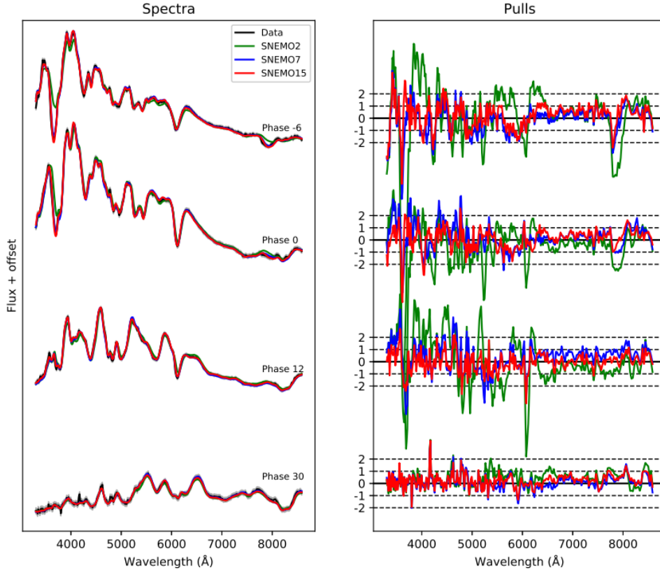
Fig. 2.15 Model reconstruction of SNEMO on SNfactory spectra ([Saunders et al., 2018]). On the left we see the fluxes of the spectra in comparison with 3 SNEMO models containing 2 (green), 7 (blue) and 15 (red) parameters. The right figures shows the weighted residuals of each model and spectrum.
