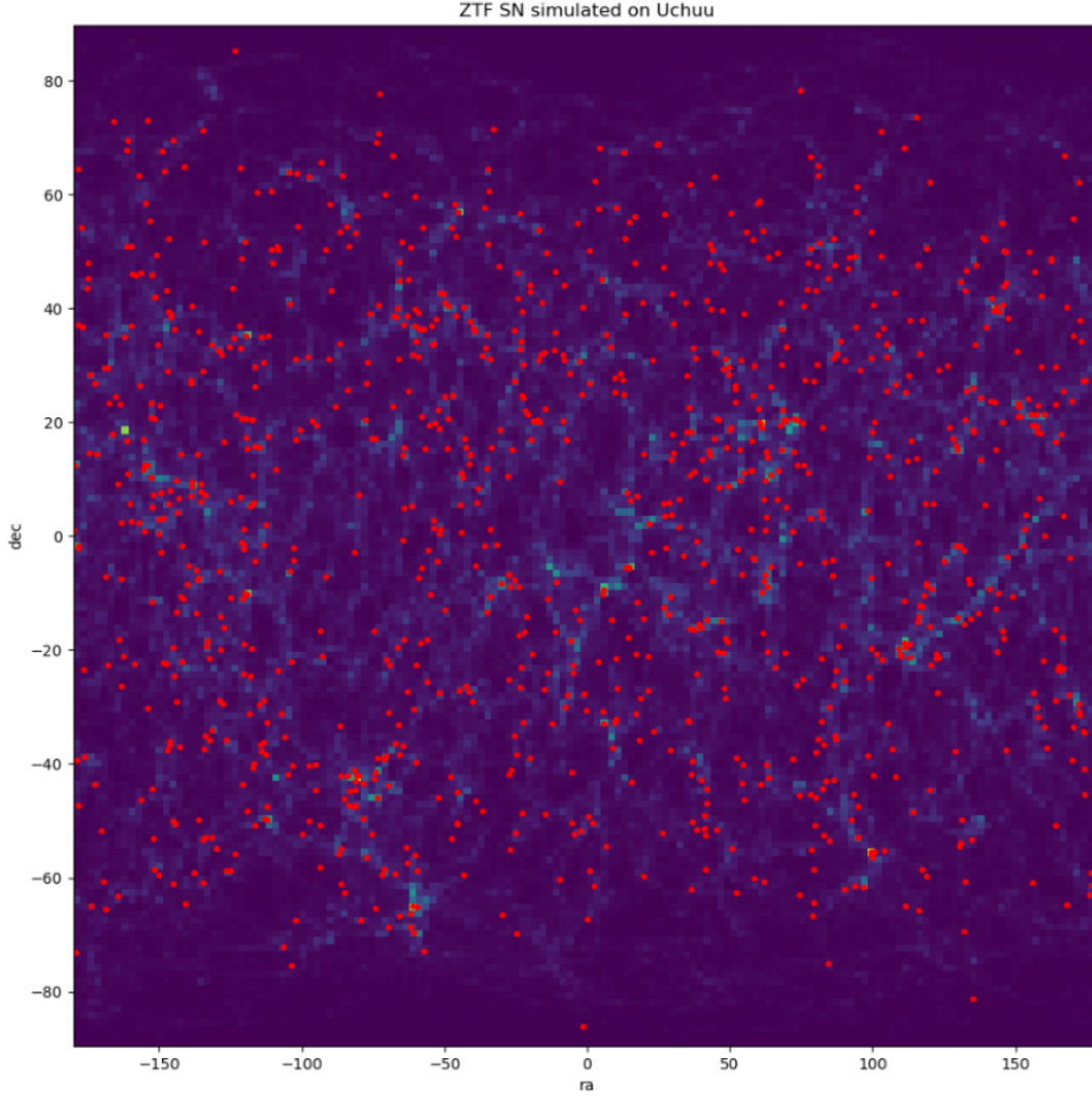
Fig. 6.2 2D full-sky projection of the Uchu density field at redshift of z \approx 0.04 with the ZTF supernovae simulated on top of it represented by red dots.
