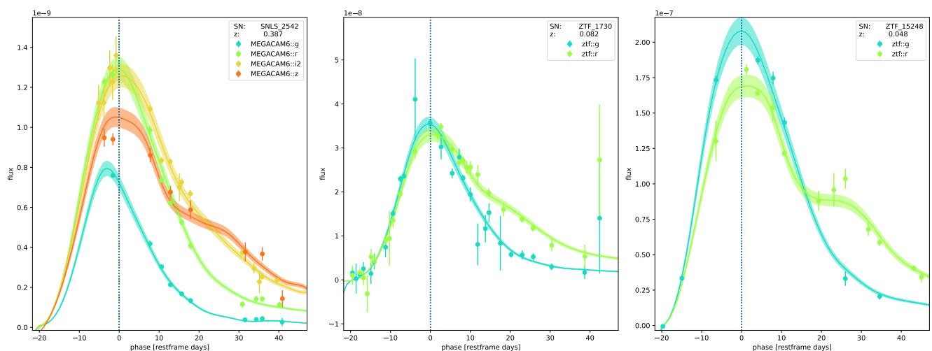
Fig. 4.1 Visual representation of the error snake on simulated lightcurves from DC1 (see section (reference)). In 4.1a we see how the model represents the data without an error snake model. In 4.1b we see a highlighted section for each lightcurves which are the variations modeled by the error snake.
