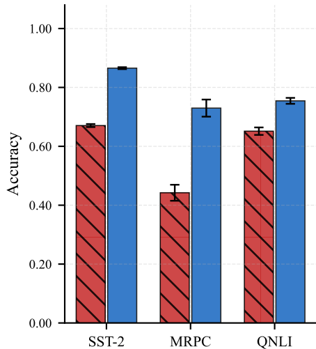
DistilBERT
