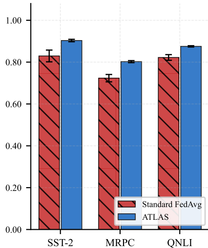
Qwen-2.5-0.5B
