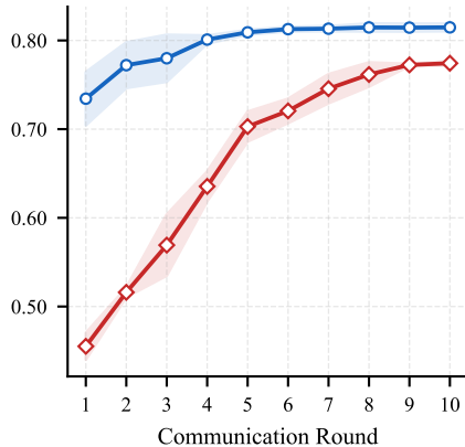
Qwen-2.5-0.5B
