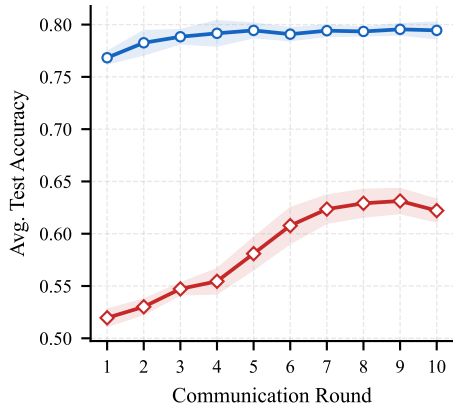
DistilBERT
