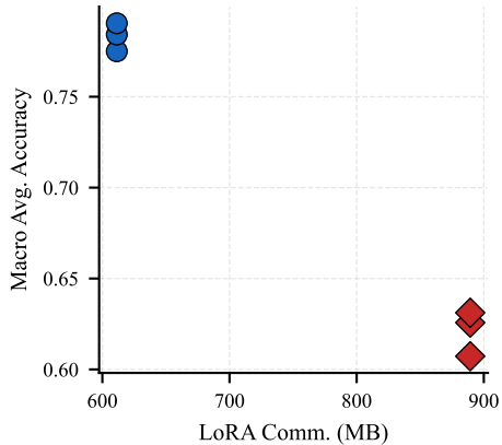
DistilBERT
