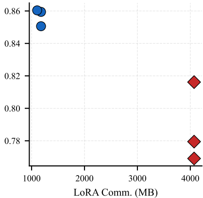
Qwen-2.5-0.5B
