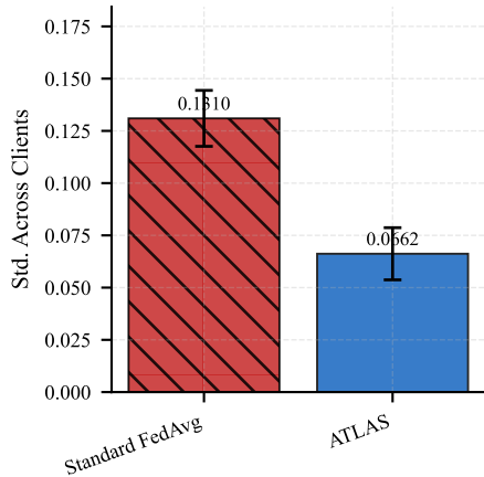
DistilBERT
