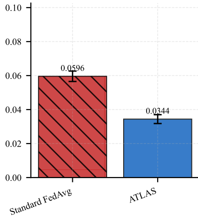
Qwen-2.5-0.5B
