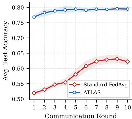
DistilBERT
