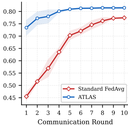
Qwen-2.5-0.5B
