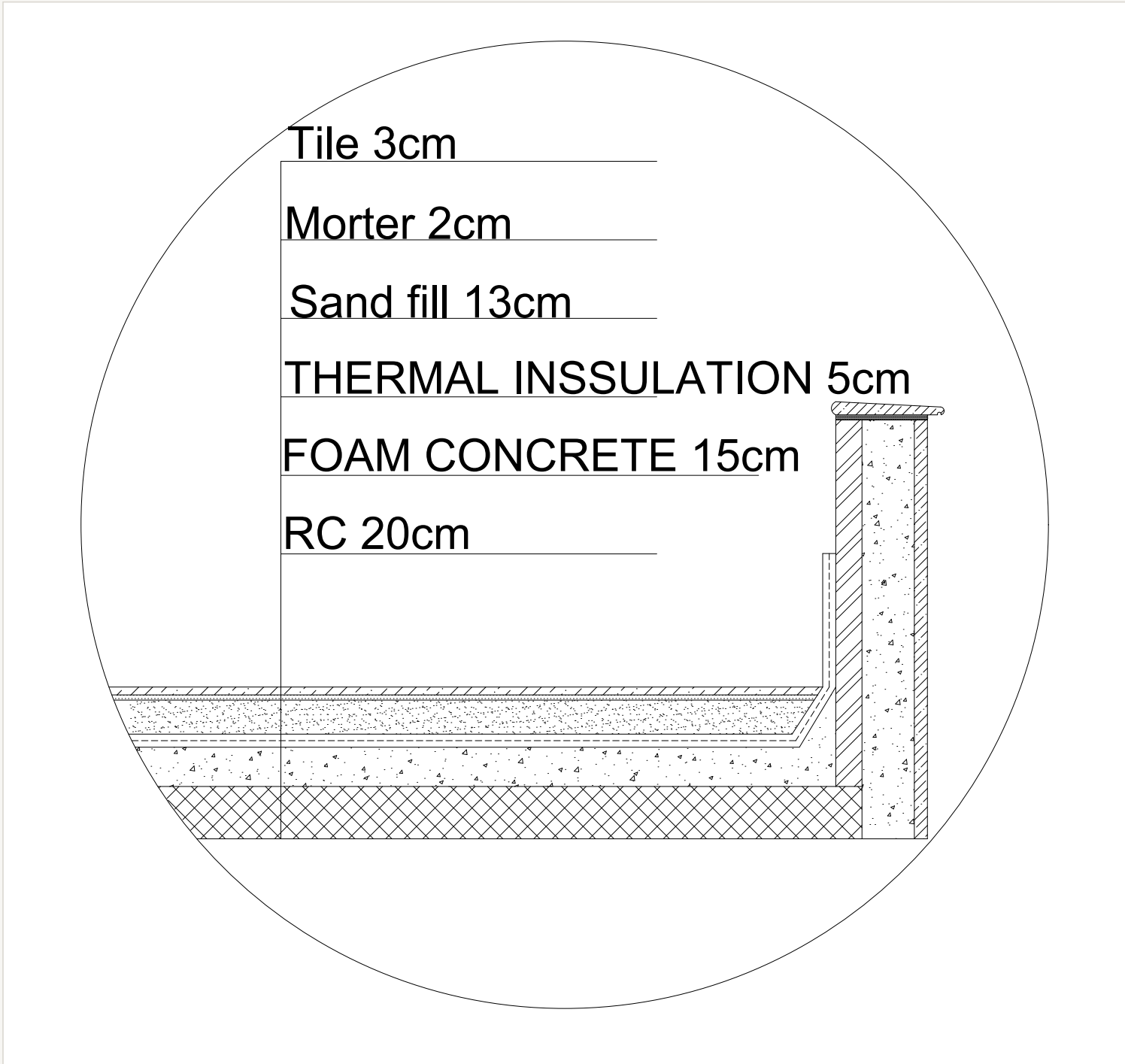
Top of roof enlargement
