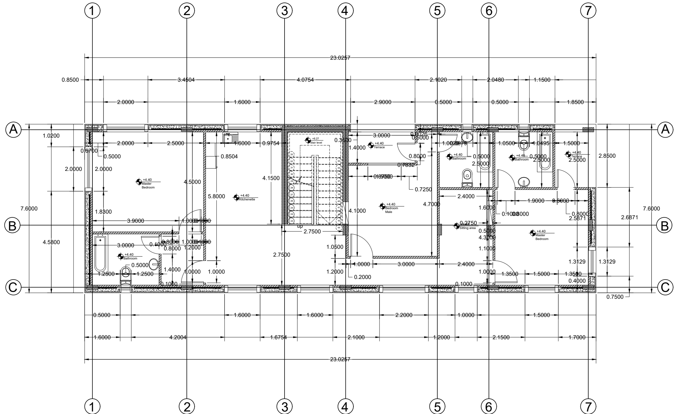
First floor – dimension plan
