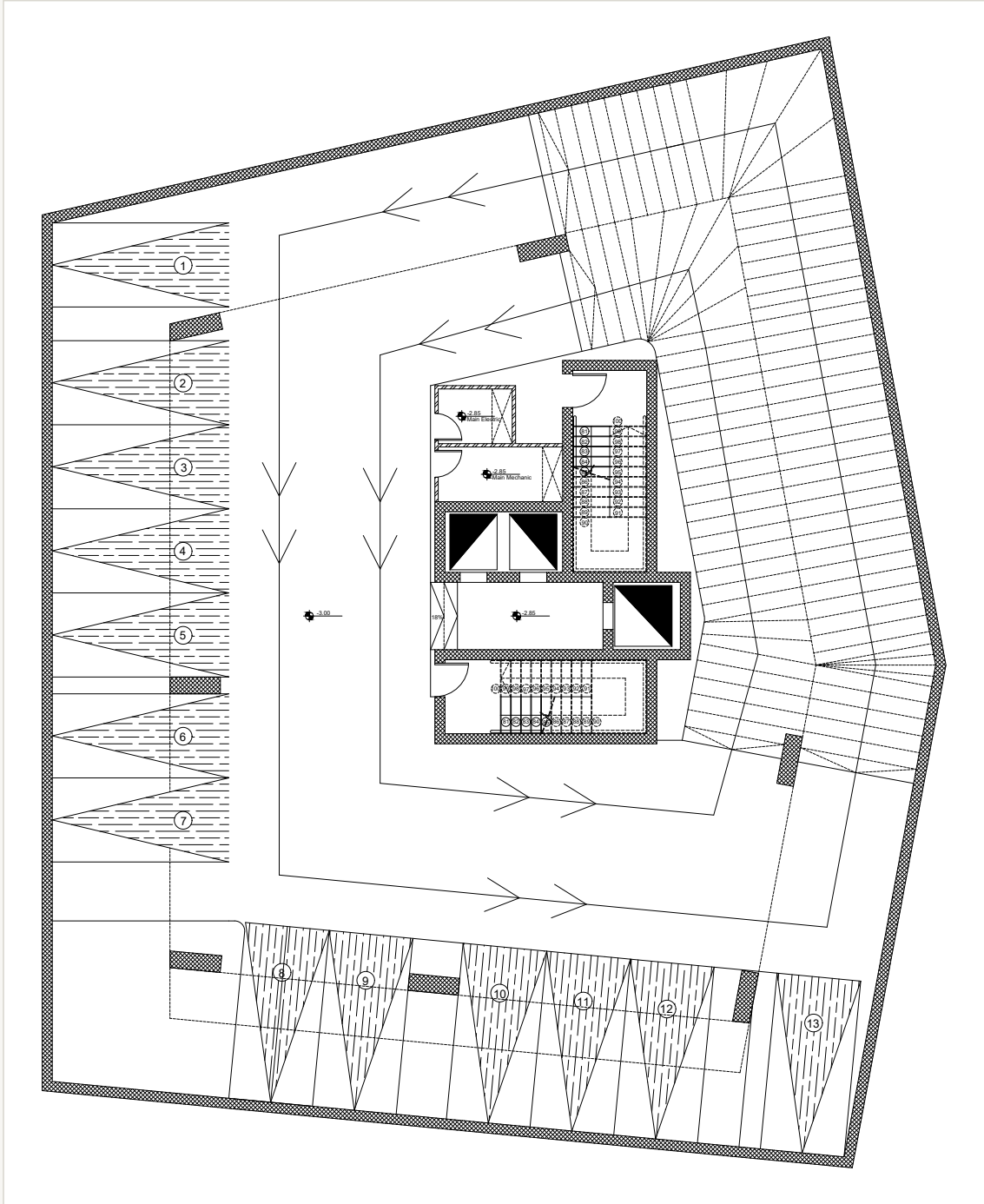
Cellar – general plan
