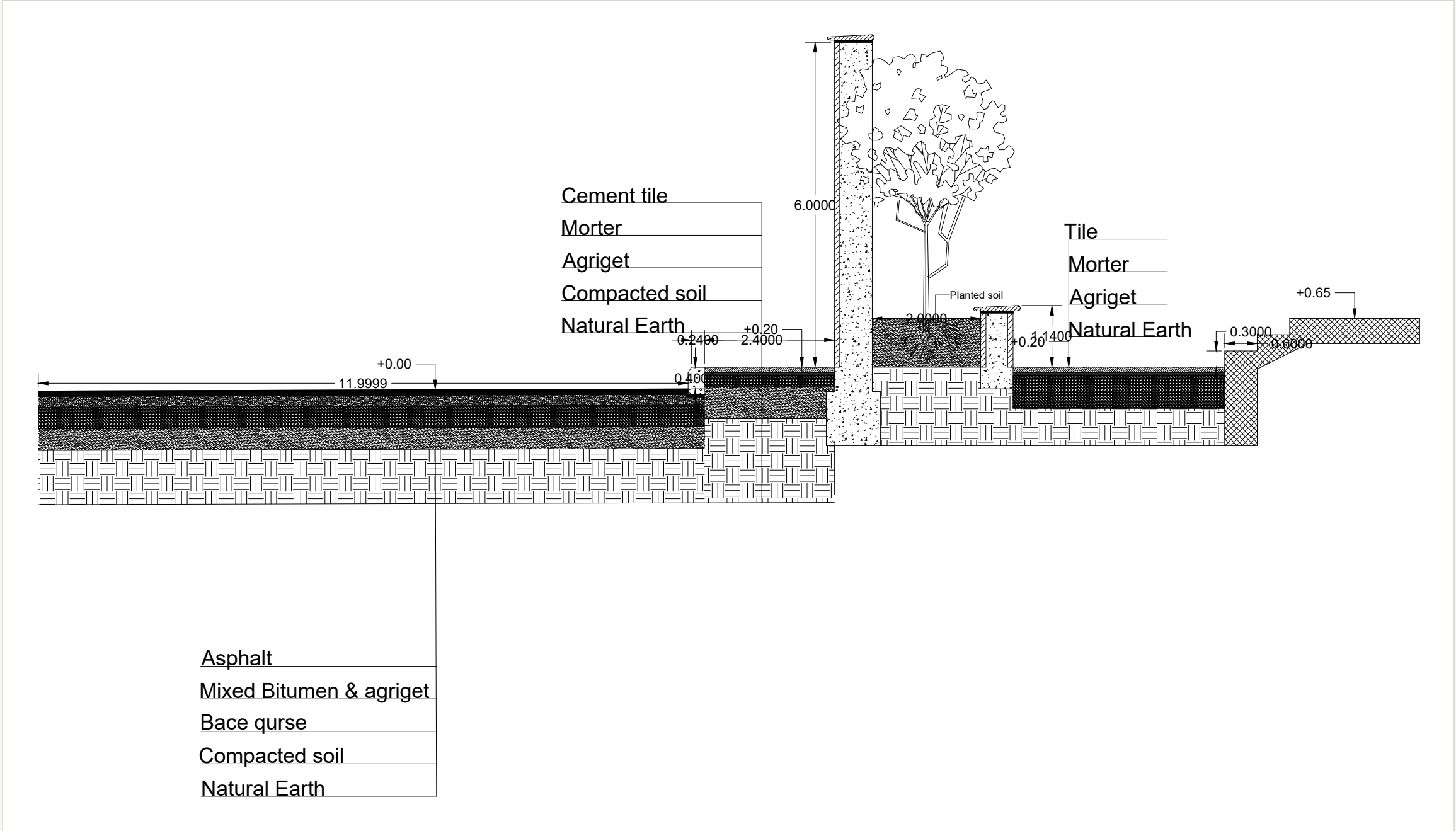
General section
