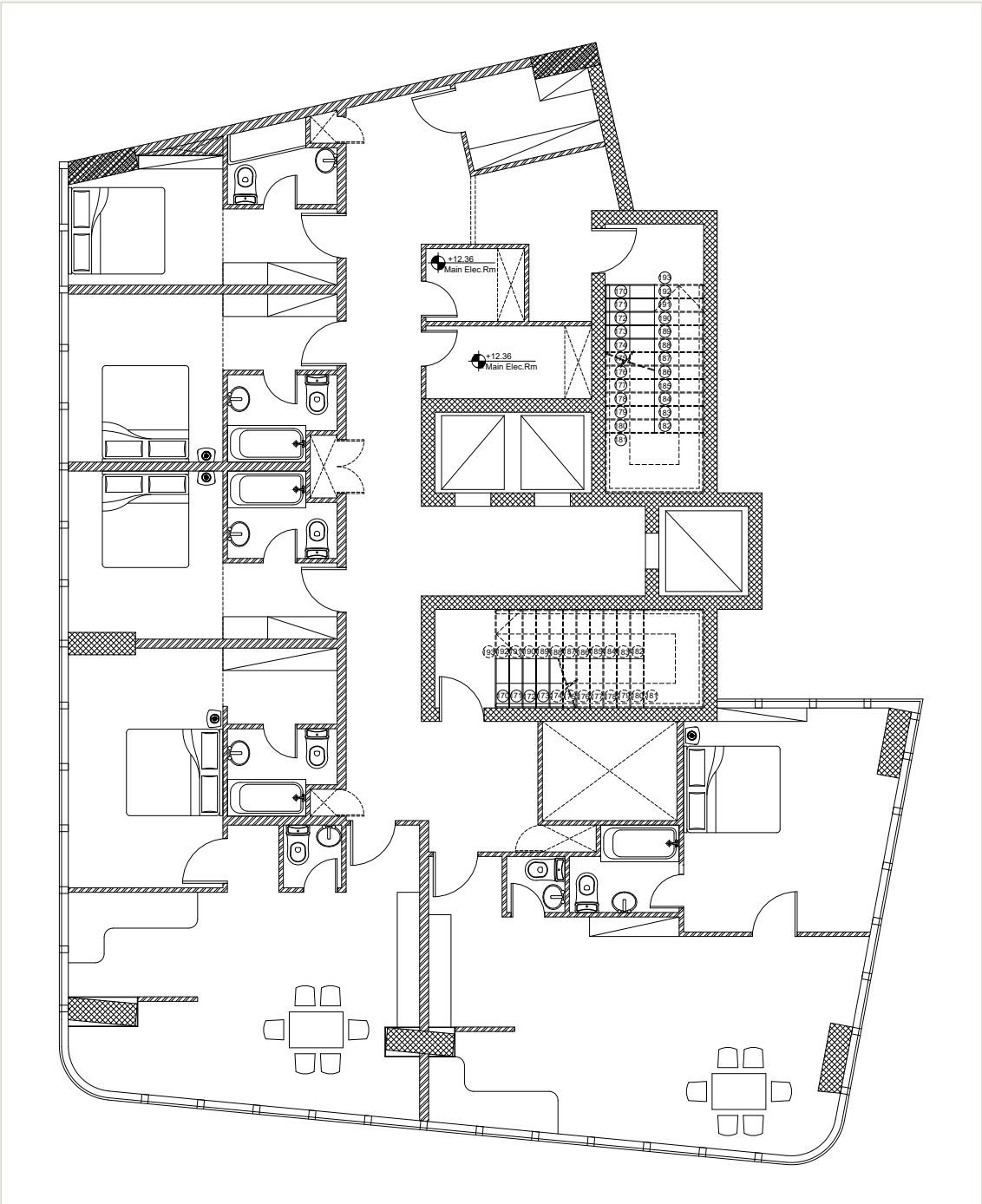
Second floor – furniture plan
