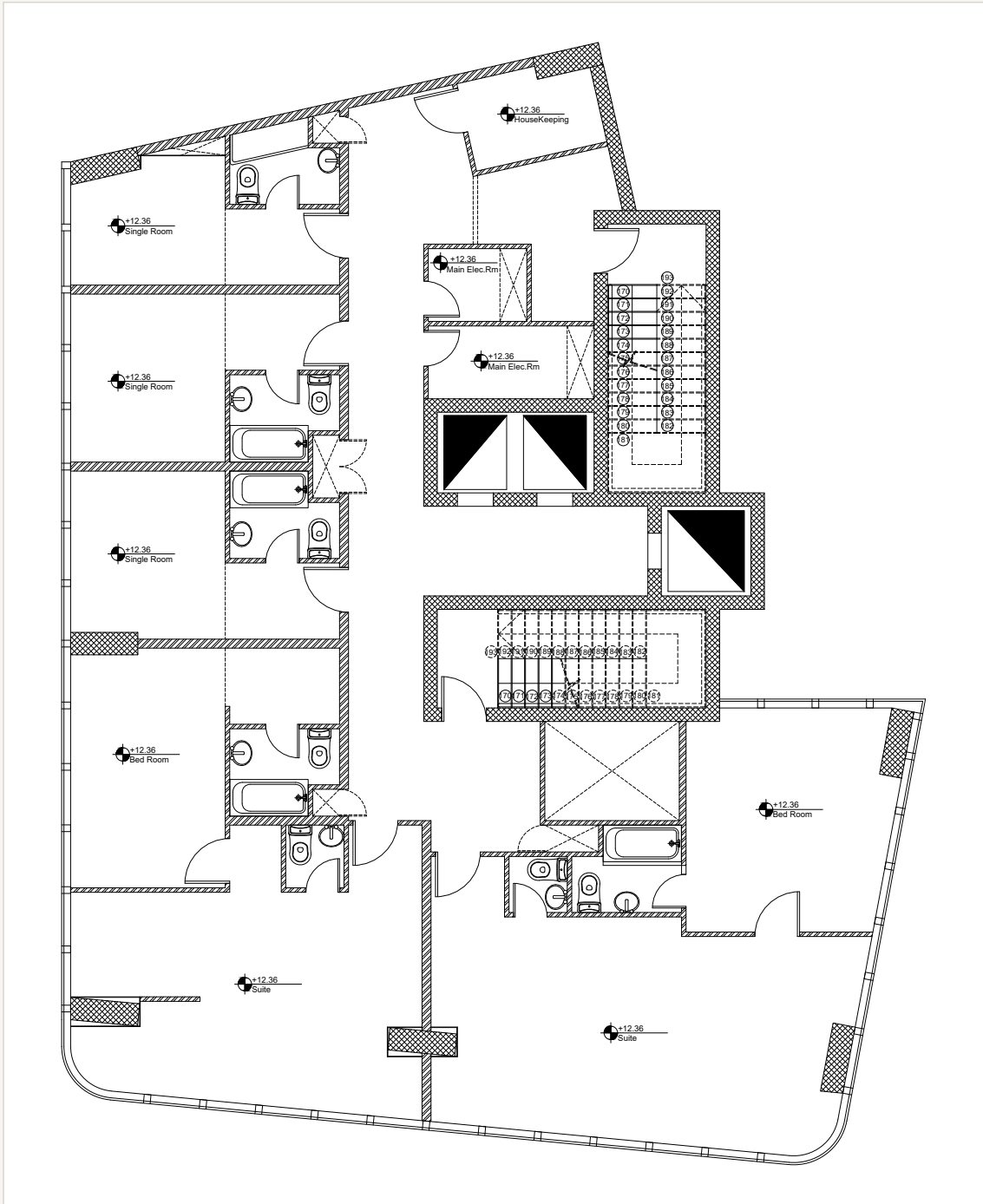
Second floor – general plan
