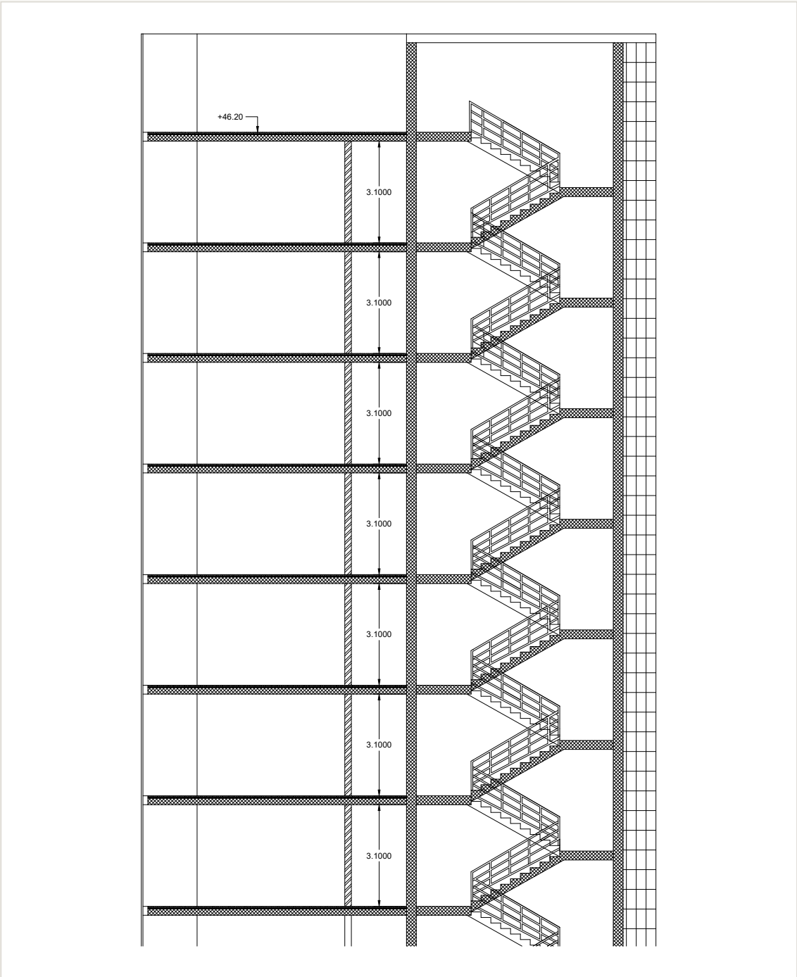
Section A-A (2/2) – upper levels
