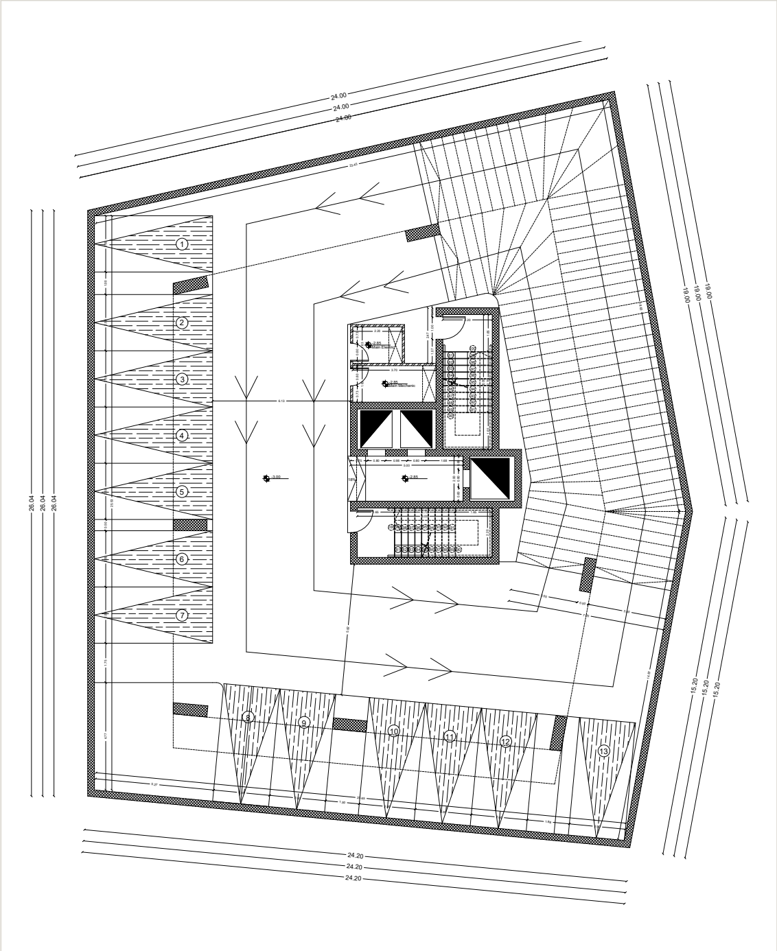
Cellar – dimension plan
