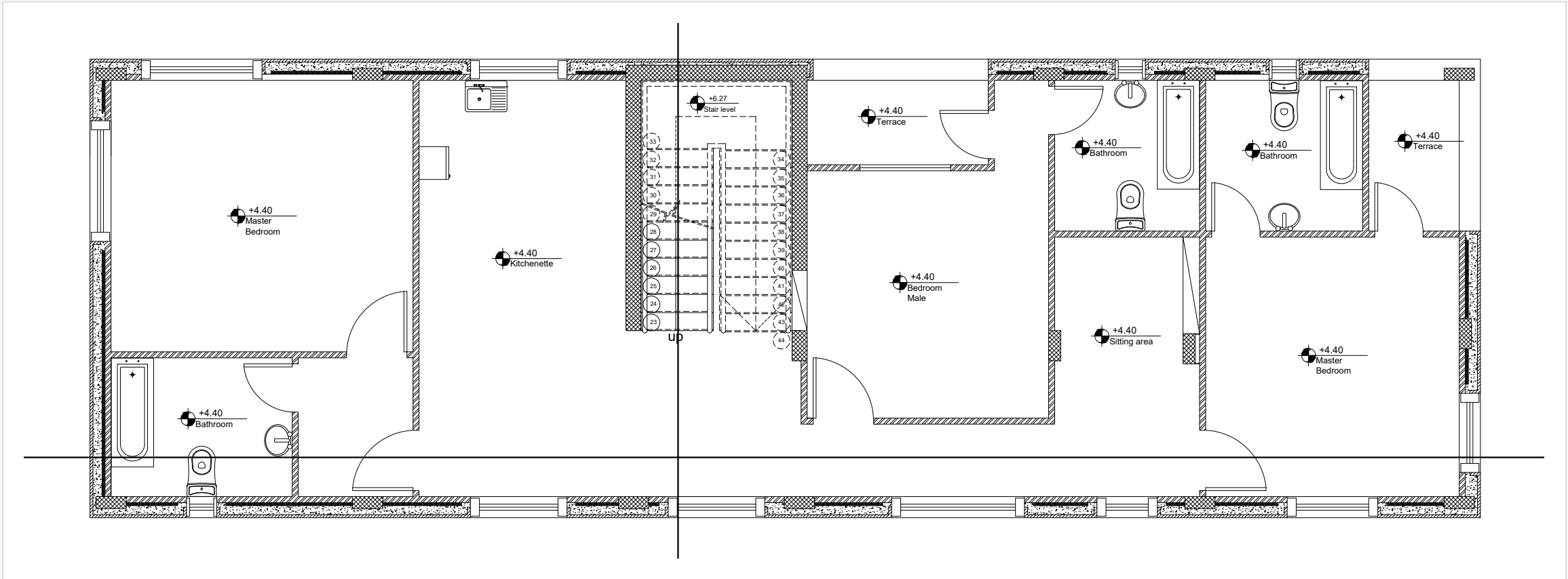
First floor – general plan
