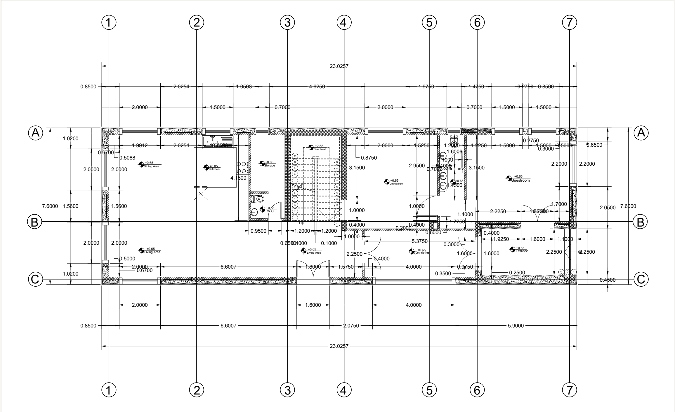
Ground floor – dimension plan
