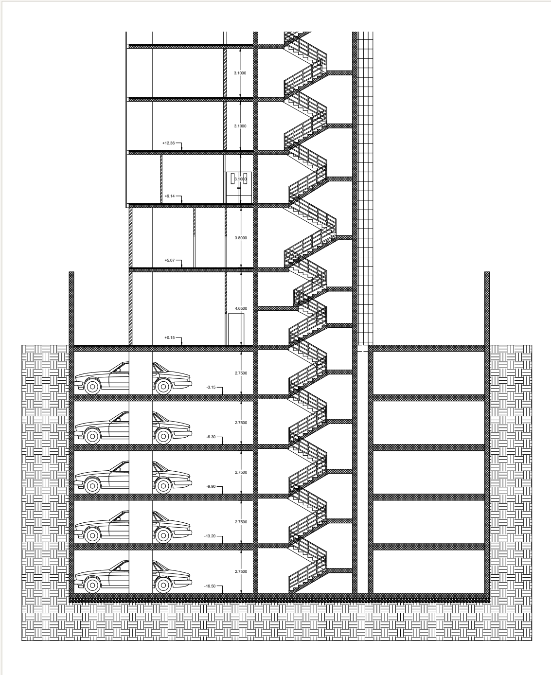
Section A-A (1/2) – cellar and lower levels
