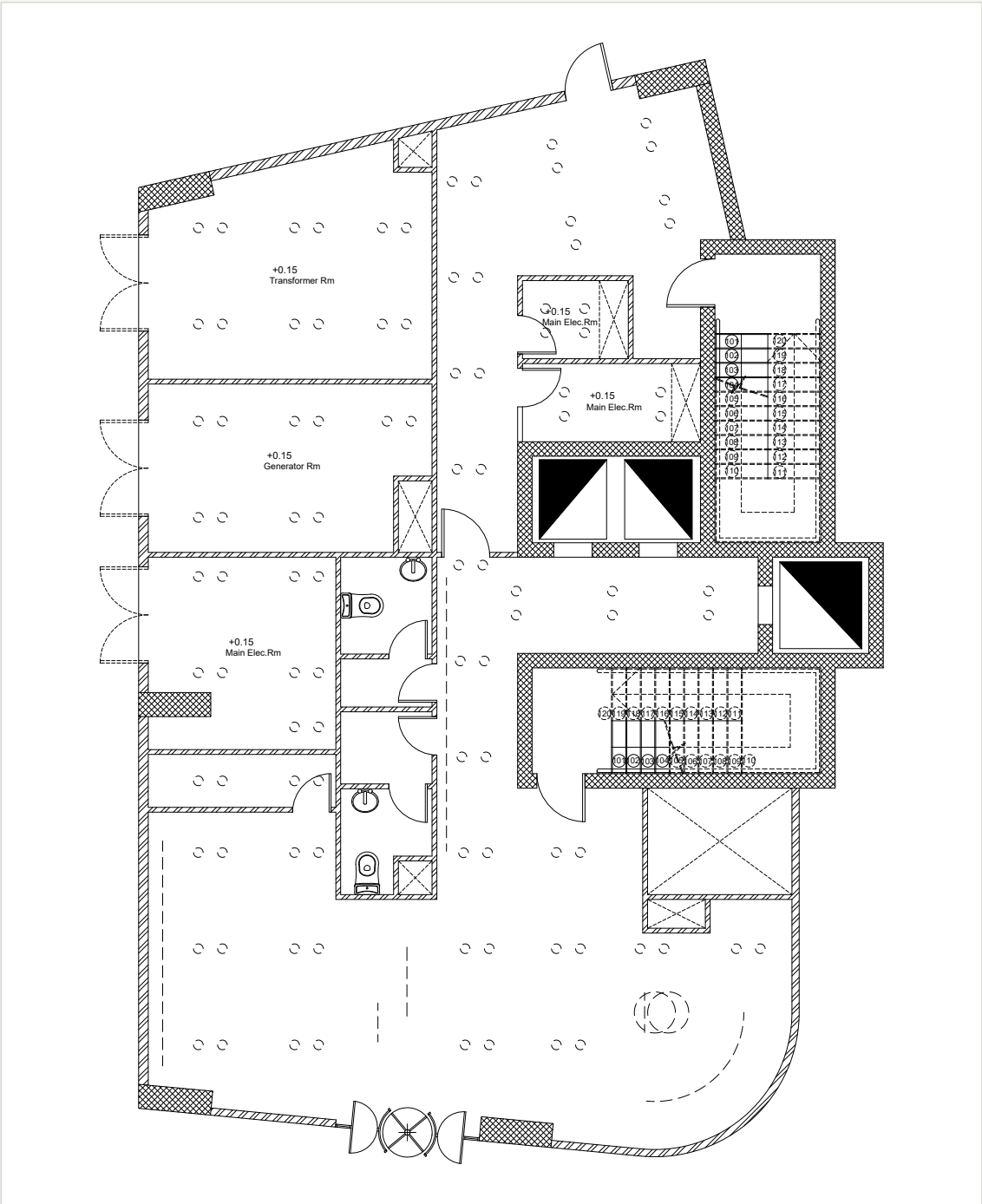
Ground floor – lighting plan
