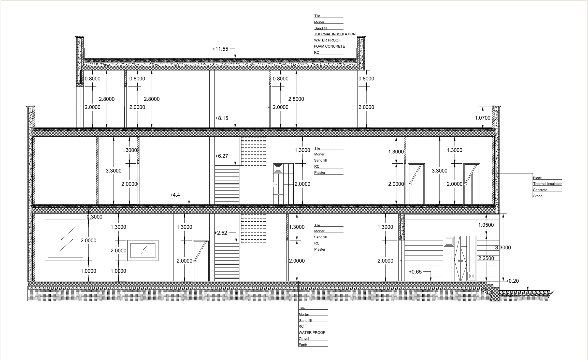
Section B-B
