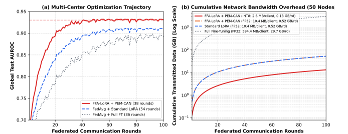
Fig. 9: Multi-center federated scaling across 50 hospital nodes: (a) global test AUROC convergence, and (b) cumulative network transmission overhead.
