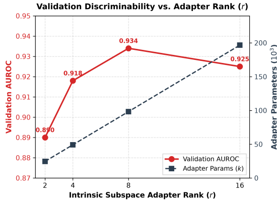
Fig. 5: Validation AUROC vs. adapter rank dimension ( r \in \{2, 4, 8, 16\} ) and adapter parameter budget.
