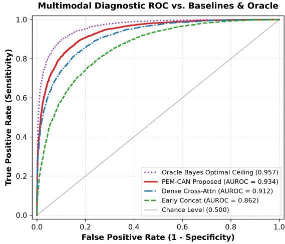
Fig. 3: Receiver Operating Characteristic (ROC) curves on the held-out test cohort comparing PEM-CAN against dense cross-attention, early concatenation, and the theoretical Oracle Bayes Optimal ceiling.
