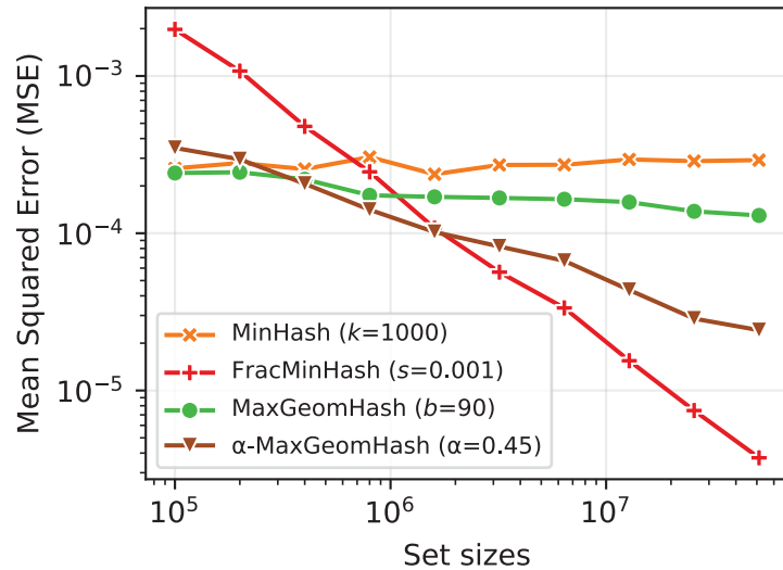
b. MSE for Jaccard
