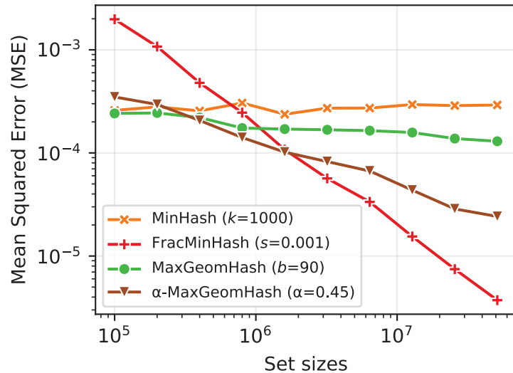
B. MSE in Jaccard estimation
