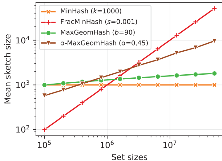
A. Average sketch sizes
