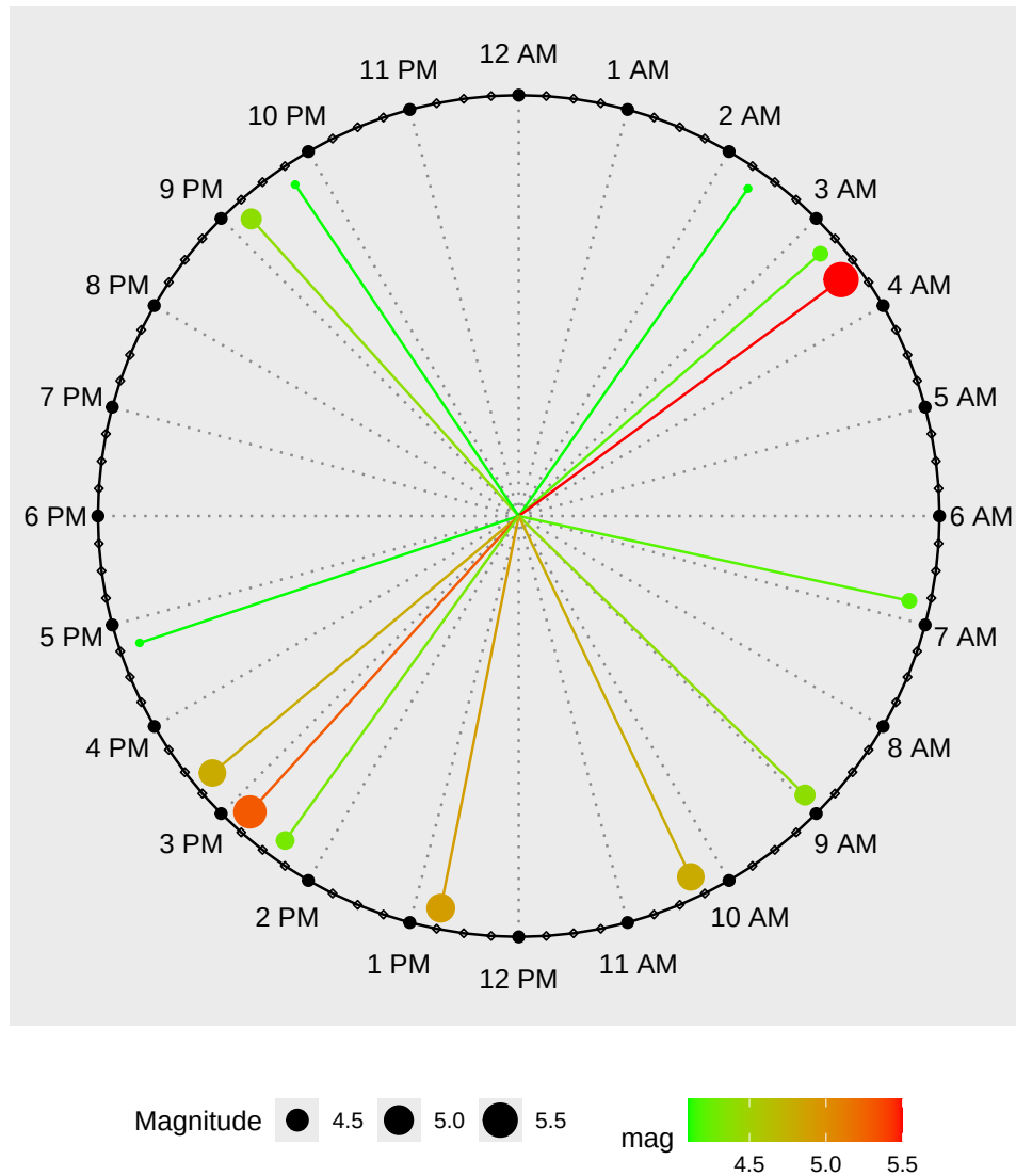
Earthquakes in Bangladesh since 2023
