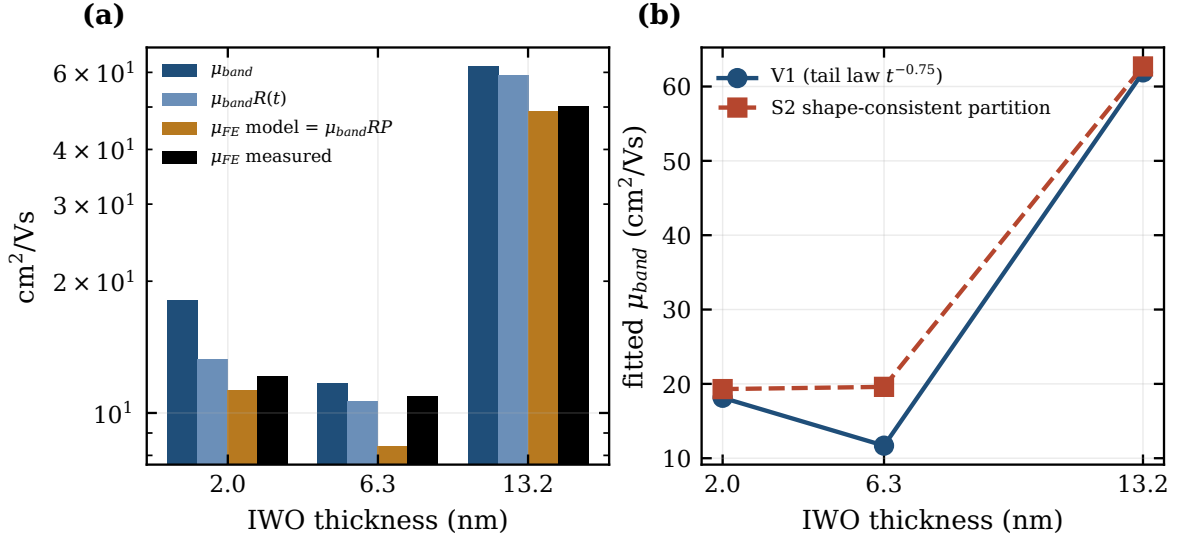
Figure 9.2. Partition of the apparent mobility, \mu_{FE} = \mu_{band} \times R(t) \times P (Equation (9.1)), per film. Left: the V1 calibration (runs run_0012 , run_0015 , run_0013 ); right: the S2 shape-consistent partition from the 1-D surrogate, \mu_{band} = 19.3/19.6/62.7 \text{ cm}^2/\text{Vs} with N_t = 2.4\text{e}19/2.7\text{e}19/4.8\text{e}18 \text{ cm}^{-3} . In both partitions the roughness factor and the partition factor change by only a few per cent between 6.3 and 13.2 nm, so the \times 4.6 step lies in \mu_{band} .
