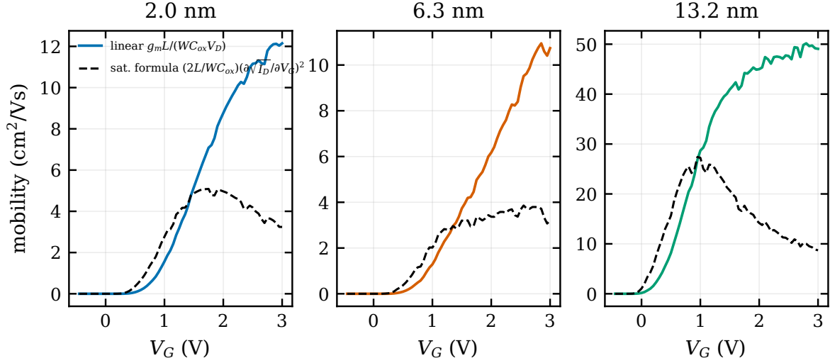
Figure 5.1. Mobility extraction from the measured transfer curves at V_D = 0.7 \text{ V} for 2.0, 6.3 and 13.2 nm. The linear-regime estimator \mu_{\text{FE}}(V_G) = Lg_m/(WC_{\text{ox}}V_D) (Equation (5.11)) is compared with the saturation formula (2L/WC_{\text{ox}})(\partial\sqrt{I_D}/\partial V_G)^2 (Equation (5.12)). Derivatives use numpy.gradient on the measured 0.05 V grid. The peaks are 12.15 / 10.95 / 50.17 cm 2 /V s (linear) against 5.09 / 3.86 / 27.40 cm 2 /V s (saturation formula). The target paper quotes 5.1 and 27.4 cm 2 /V s for 2 and 13.2 nm. Note that the 2 nm linear estimator is still rising at the end of the sweep.
