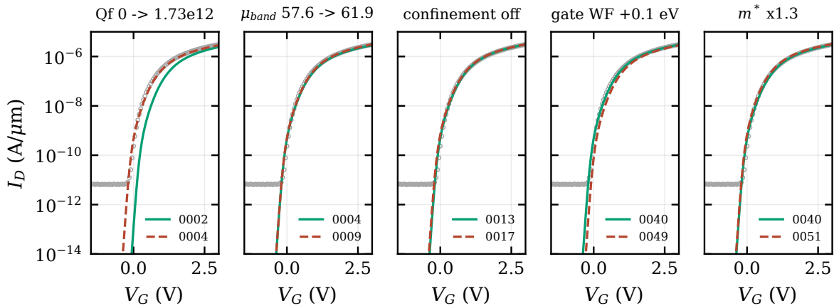
Figure 7.6. Parameter control at 13.2 nm: Q_f 0 \rightarrow 1.73 \times 10^{12} \text{ cm}^{-2} (run_0002→run_0004), \mu_{band} 57.6 \rightarrow 61.9 (run_0004→run_0009), confinement off (run_0017 vs run_0013), gate WF +0.1 eV (run_0049 vs run_0040) and m^* \times 1.3 (run_0051 vs run_0040), against the measured 13.2 nm curve. Switching confinement off changes the 13.2 nm threshold by only -23 mV, against -316 mV at 2 nm.
