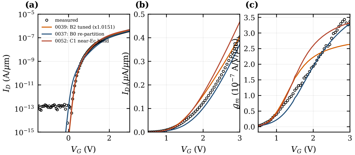
Figure 8.3. The 6.3 nm on-state shape: measured curve against B2 (run_0039, rescaled by 11.581987/11.41), B0 (run_0037, tail re-partition) and C1 (run_0052, near- E_c acceptor band). (a) \log_{10} I_D ; (b) linear I_D ; (c) g_m(V_G) from the numerical gradient on the 0.05 V grid. B0 reproduces the on-state (b, c) but not the subthreshold region (a); C1 retains the subthreshold behaviour and recovers only part of the delayed, steep rise; B2 rises too early and too slowly.
