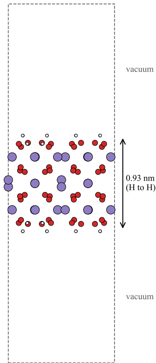
(a) 1 nm slab, relaxed \text{In}_{24}\text{O}_{48}\text{H}_{24} , 96 atoms
