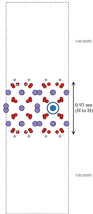
(c) 1 nm IWO slab, as built \text{In}_{23}\text{WO}_{48}\text{H}_{24}
