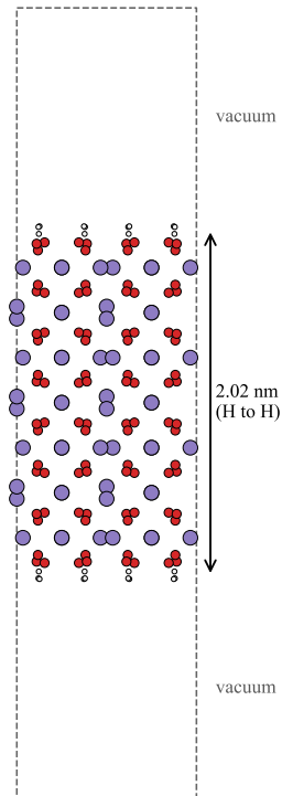
(b) 2 nm slab, as built \text{In}_{56}\text{O}_{96}\text{H}_{24} , 176 atoms
