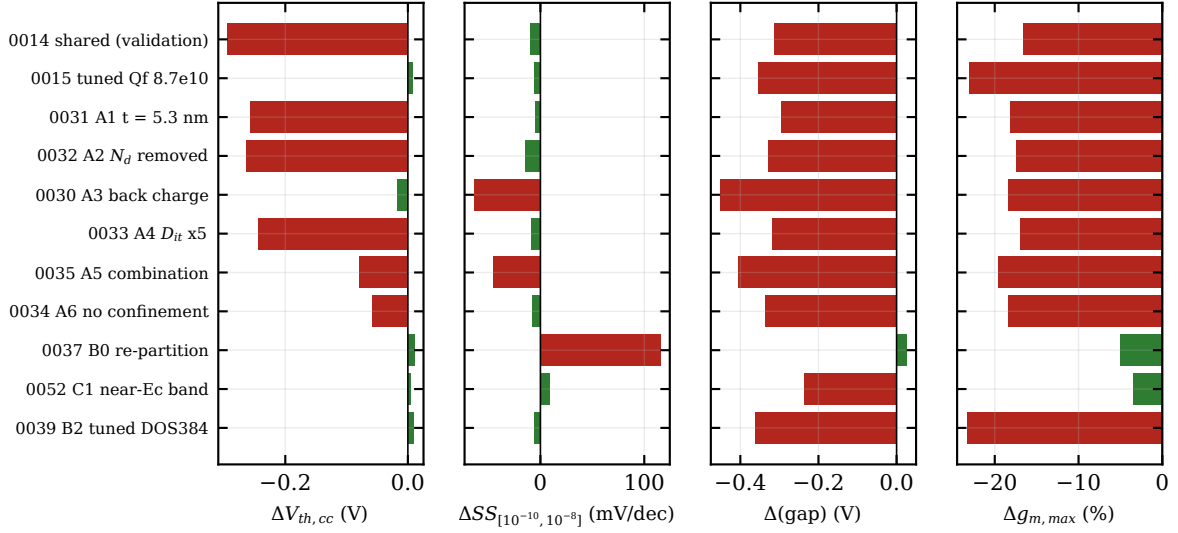
Figure 8.2. Errors of every 6.3 nm hypothesis relative to the measurement ( V_{th,cc} 0.644 V, SS_{cc} 295.4 mV/dec, gap 1.176 V, g_{m,max} 3.431 \times 10^{-7} A/V/ \mu\text{m} ); green marks agreement within 0.05 V / 20 mV/dec / 0.1 V / 8 %. V_{th,cc} , SS_{cc} , gap and g_{m,max} errors: run_0014 -0.294 V, -10.4 , -0.314 V, -16.6 %; run_0015 +0.007 V, -6.5 , -0.356 V, -23.1 %; A1 run_0031 -0.258 V, -4.9 , -0.297 V, -18.1 %; A2 run_0032 -0.264 V, -14.7 , -0.329 V, -17.5 %; A3 run_0030 -0.017 V, -64.1 , -0.452 V, -18.4 %; A4 run_0033 -0.243 V, -9.1 , -0.319 V, -16.9 %; A5 run_0035 -0.079 V, -45.9 , -0.405 V, -19.6 %; A6 run_0034 -0.057 V, -7.7 , -0.337 V, -18.4 %; B0 run_0037 +0.010 V, +115.6 , +0.026 V, -5.0 %; C1 run_0052 +0.004 V, +9.1 , -0.237 V, -3.5 %; B2 run_0039 +0.009 V, -5.7 , -0.362 V, -23.3 %. No case is green in all four metrics.
