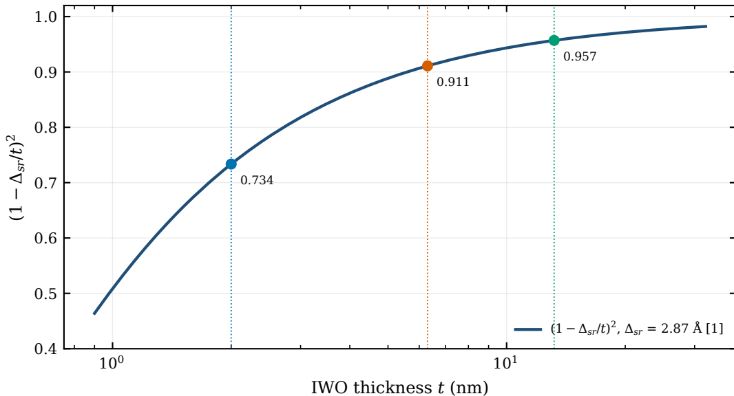
(e) Surface-roughness mobility factor, model V1
