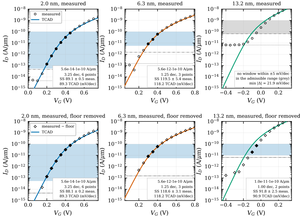
Post hoc, descriptive. One-decade windows with |\text{SS}_{\text{TCAD}} - \text{SS}_{\text{meas}}| \leq 5 mV/dec, upper edge \leq 10^{-9} A/ \mu\text{m} ; lower edge \geq 10 \times floor (top row) or \geq 1 \times floor (bottom row, assumes an additive, gate-independent floor). Dotted: measured floor; dash-dot: lowest admissible edge. Filled symbols: measured points inside the agreement range.
