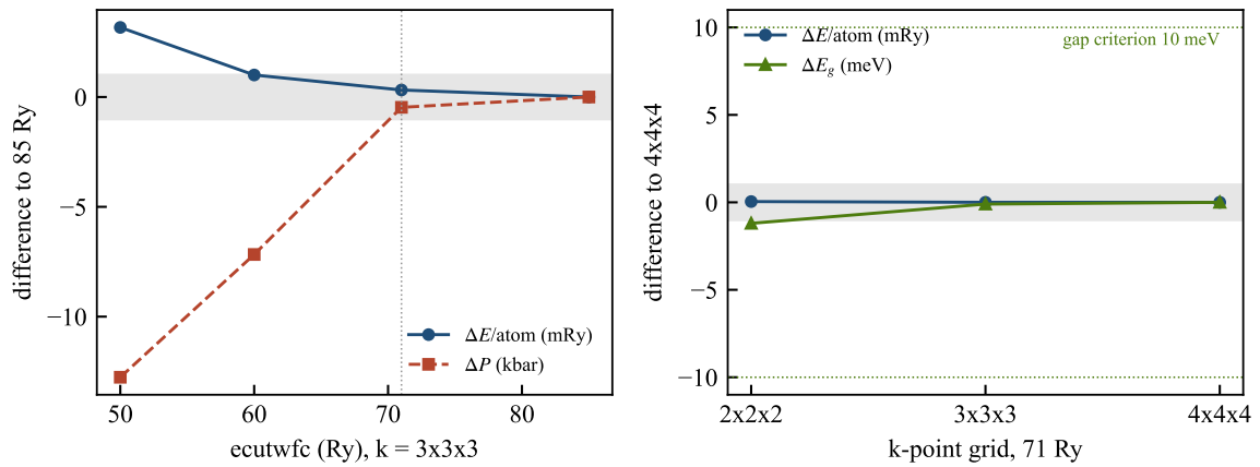
Figure 12.7. Convergence of total energy, pressure and Kohn–Sham gap of bulk \text{In}_2\text{O}_3 with the plane-wave cutoff (left, 3 \times 3 \times 3 ) and the k -point grid (right, 71 Ry). The grey band marks the energy criterion of 1 mRy per atom; the dotted lines on the right mark the gap criterion of 10 meV.
