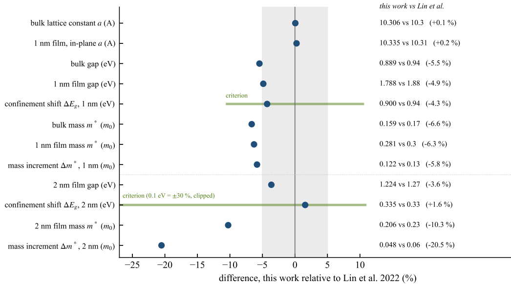
Figure 12.11. This work against the PBE calculations of Lin et al. [1, pp. 21540, 21542], which used the same slab recipe: relative difference of each quantity (dots) with both values written out. Grey: \pm 5\% ; green: the pre-registered tolerance of the confinement shift ( \pm 0.1 eV; at 2 nm this is \pm 30\% and the bar is clipped). For the in-plane lattice constant of the 1 nm film, Lin et al. give 10.26 and 10.36 Å; their mean is compared with ours. Below the dotted line: the 2 nm film (Section 12.5.11); no criterion was set for the masses. The increments of Lin et al. are differences of their rounded values ( 1.27 - 0.94 eV and 0.23 - 0.17 m_0 ).
