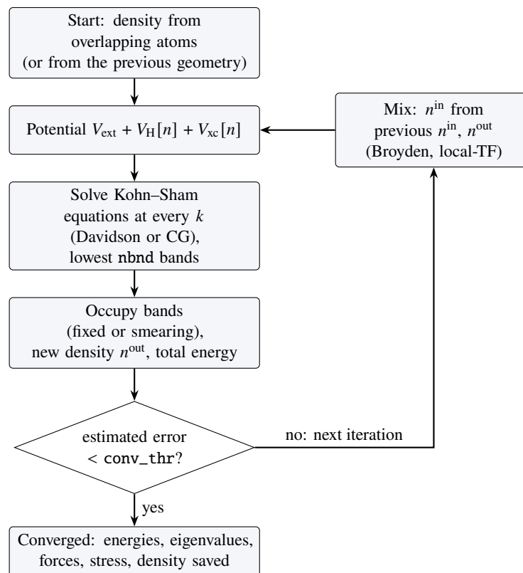
Figure 12.2. The self-consistent field (SCF) loop of a Kohn–Sham calculation, as implemented in Quantum ESPRESSO [3, pp. 13–15]. In this study the loop stops at an estimated energy error of 10^{-9} Ry; it takes 25 iterations for the bulk cell and 47 for the relaxed 1 nm slab.
