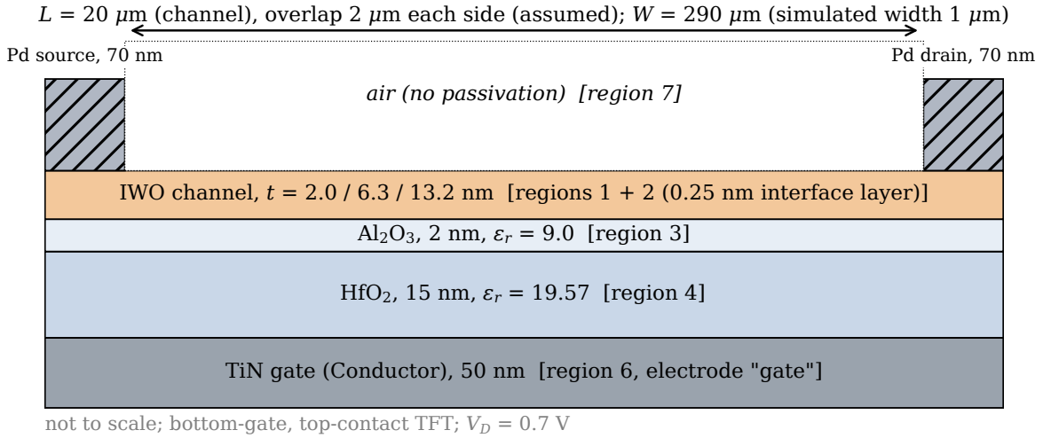
Figure 3.1. Cross-section of the modelled device (not to scale): TiN gate 50 nm, \text{HfO}_2 15 nm, \text{Al}_2\text{O}_3 2 nm, IWO channel of thickness t , Pd source/drain 70 nm overlapping the channel by 2 \mu\text{m} on each side, air above the channel; L = 20 \mu\text{m} , W = 290 \mu\text{m} . The ATLAS region numbers of the physical-structure deck are indicated (1: IWO bulk; 2: 0.25 nm IWO interface layer; 3: \text{Al}_2\text{O}_3 ; 4: \text{HfO}_2 ; 6: Conductor gate volume; 7: Air). Drawn from config/geometry.yaml and docs/DEVICE_STRUCTURE.md.
