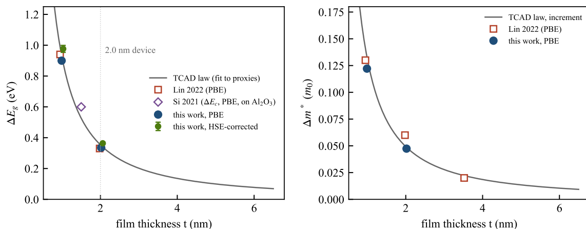
Figure 12.15. Confinement shift (left) and mass increment (right) versus film thickness: thickness laws of the device model, PBE slab values of Lin et al. [1, pp. 21540, 21542], the conduction-band shift of Si et al. [2, p. 504] (corundum \text{In}_2\text{O}_3 on \text{Al}_2\text{O}_3 , PBE), and this work (PBE, and the HSE06-corrected range of Section 12.5.8, drawn slightly offset in thickness for visibility). Thickness of this work: H–H distance of the slab as built (0.99 and 2.02 nm). The HSE06 correction measured at 1 nm is applied unchanged at 2 nm (an assumption, not a calculation).
