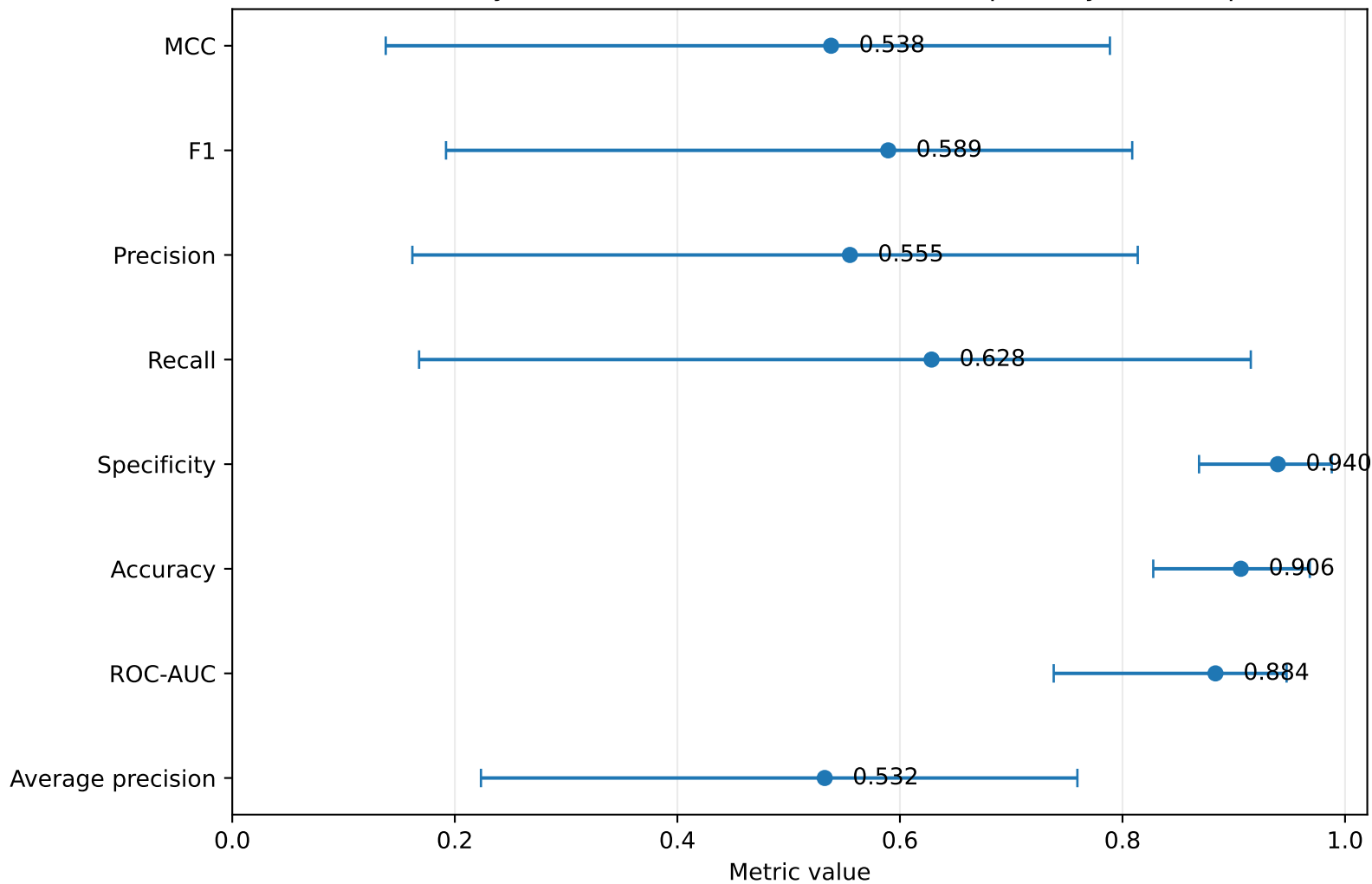
Gate 5 Binary Confirmation Metrics with 95% Repository-Bootstrap CI
