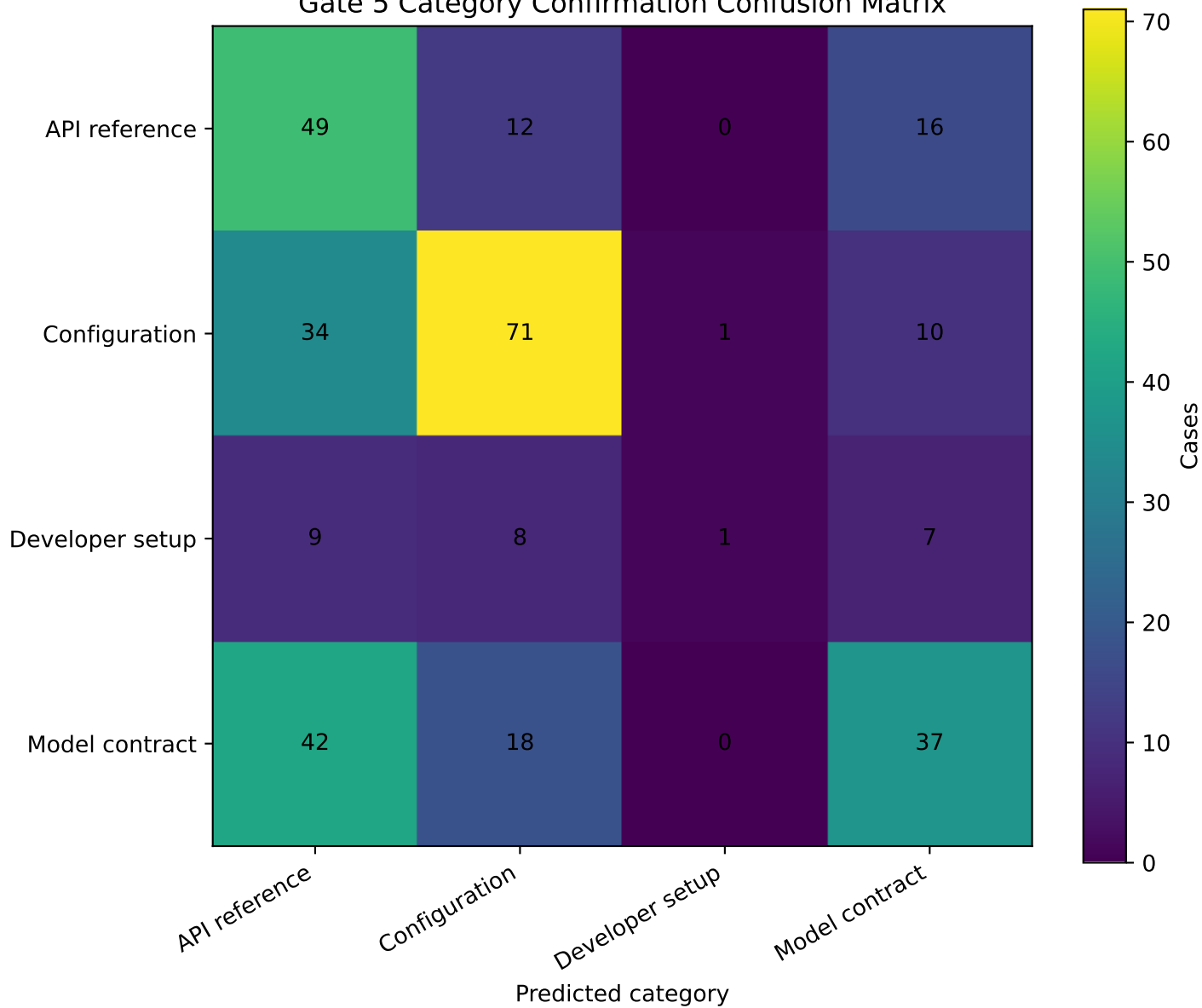
Gate 5 Category Confirmation Confusion Matrix
