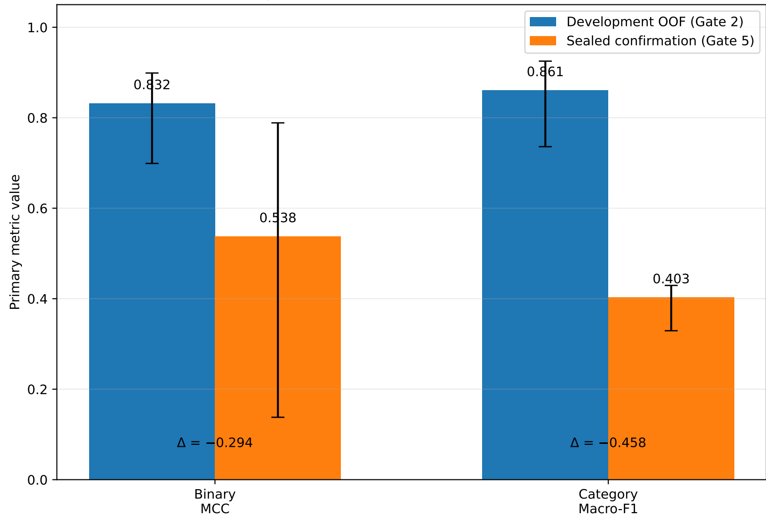
Development vs. Sealed Confirmation Performance
