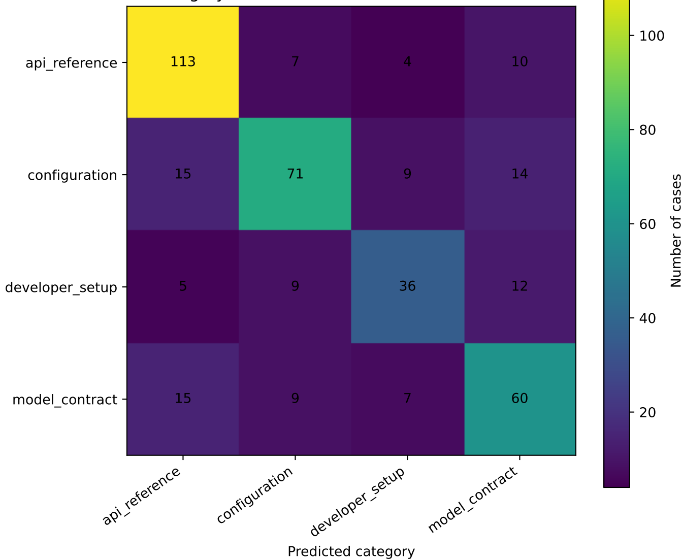
Category classifier confusion matrix — validation
