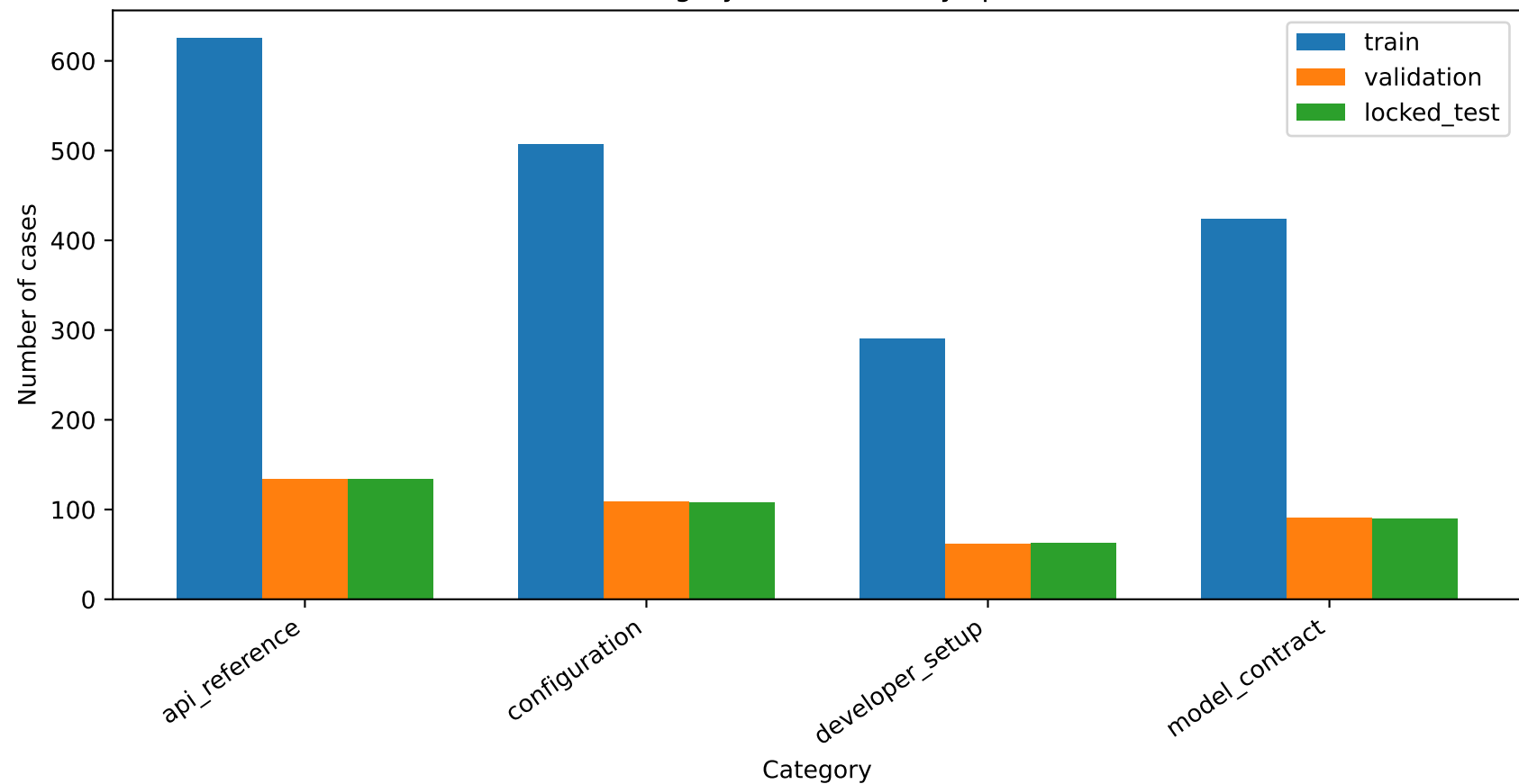
Category distribution by split
