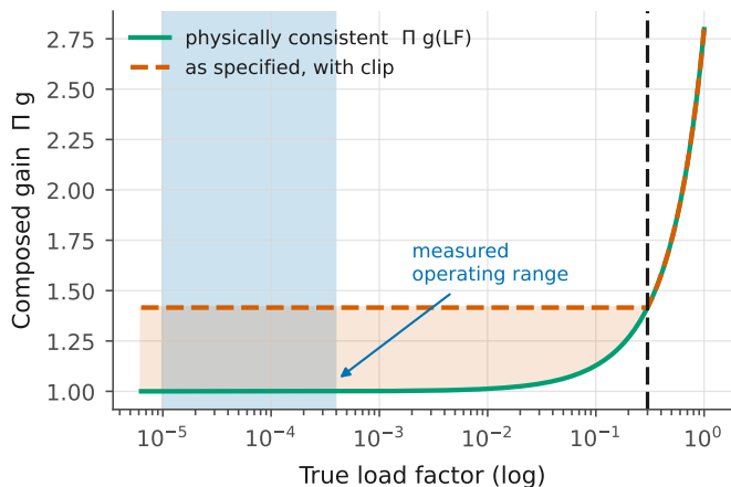
(b) Gain manufactured by the clip
