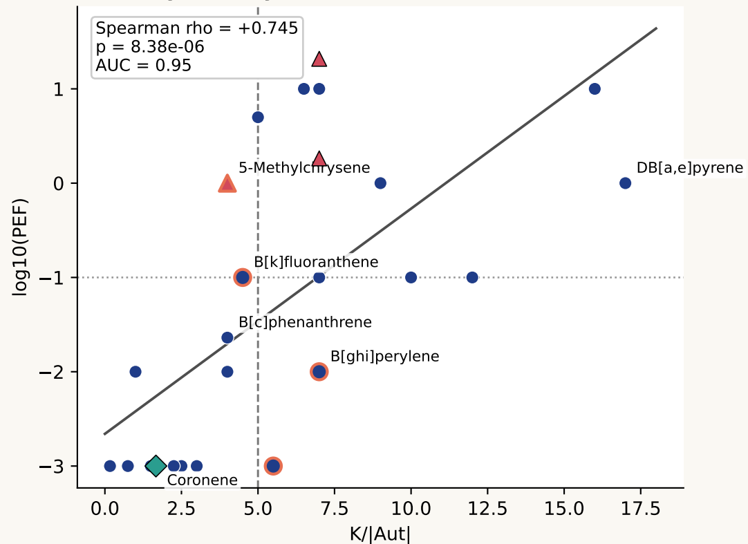
B. Symmetry-Corrected Localization Index
