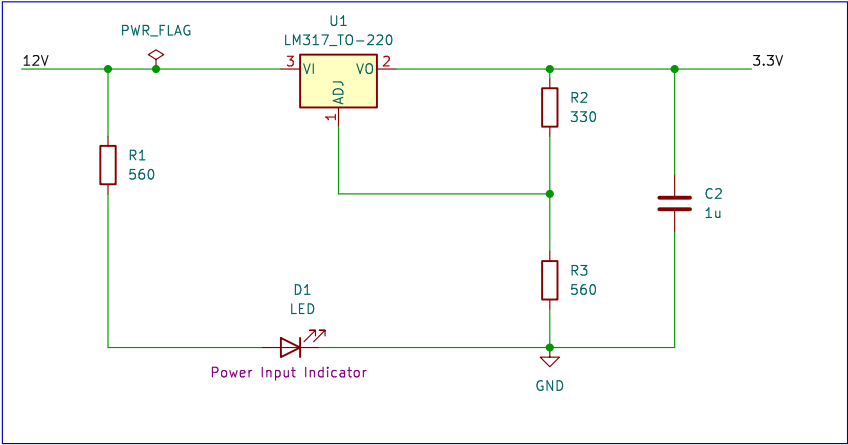
3.3V Circuit
