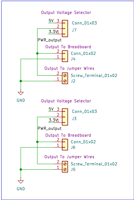
Output and Switches
