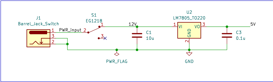
Input and 5V Circuit
