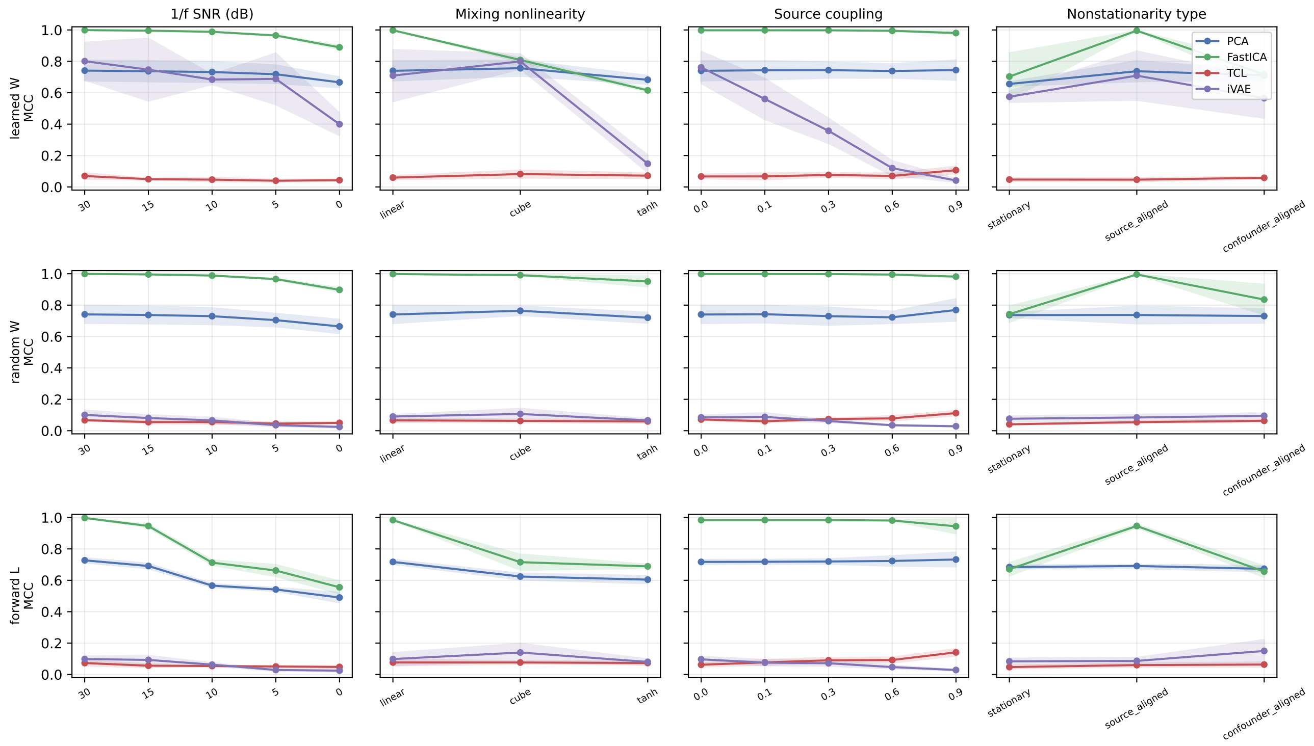
Failure axes under three mixing generators (shared source dynamics)
