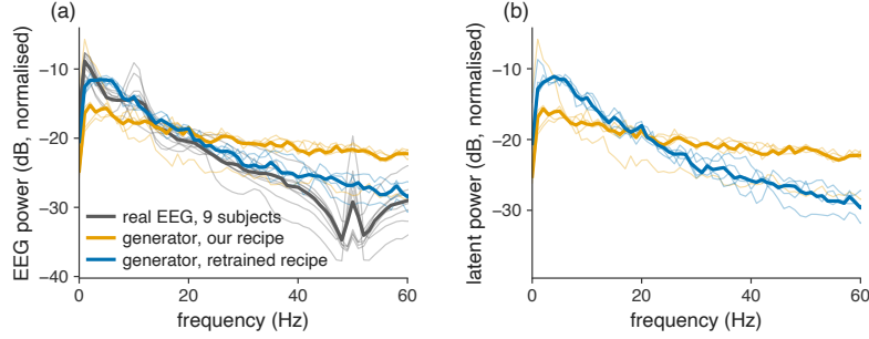
Figure 6: (a) Normalised power spectra of real BCI IV-2a EEG (per subject) and of the generator’s synthetic EEG W_z (per seed) for the recipe of Appendix A and for a recipe with a generalised-teacher-forcing floor of 0.2 and hidden width 64; (b) the corresponding latent spectra. Thin lines: individual subjects or seeds; thick: median.
