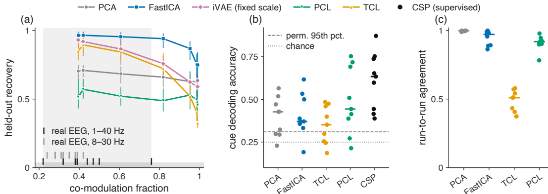
Figure 4: Real EEG. (a) The nine BCI IV-2a subjects placed on the modulation axis of Figure 2d by their observed co-modulation fraction (ticks: 1–40 Hz dark, 8–30 Hz light; shaded: their 1–40 Hz range), against the held-out recovery of the benchmark along the same axis (mean and bootstrap 95% interval over 5 seeds). (b) Four-class cue decoding accuracy from the per-trial log-variance of unsupervised components fit without labels on three runs and scored on the other three; one point per subject, bar at the median, label-permutation 95th percentile dashed, chance dotted; supervised CSP is the label-aware ceiling. (c) Agreement between the same method fit on different runs. Protocols in Appendix G.
