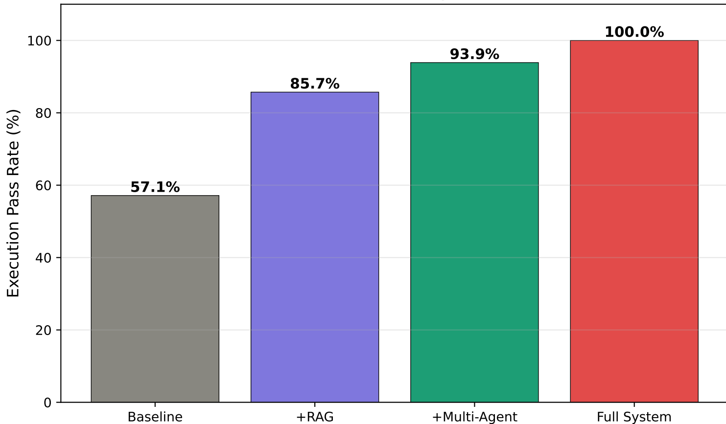
Pass Rate Across All Configurations (n=49)
