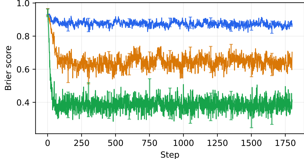
large_filter_walls: brier
