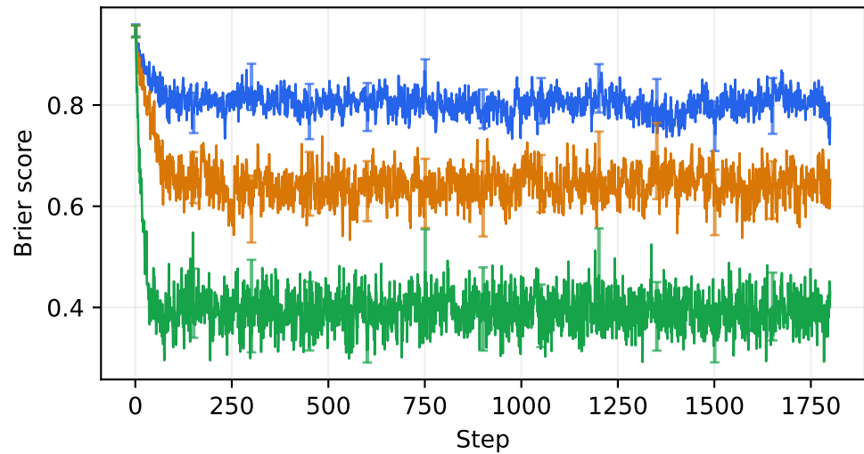
large_filter_walls: brier
