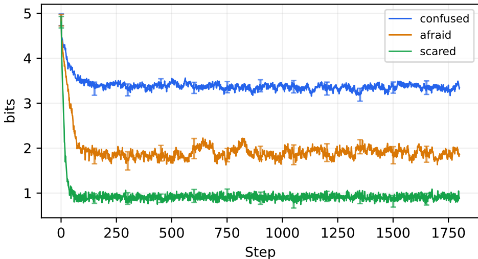
large_filter_walls: entropy
