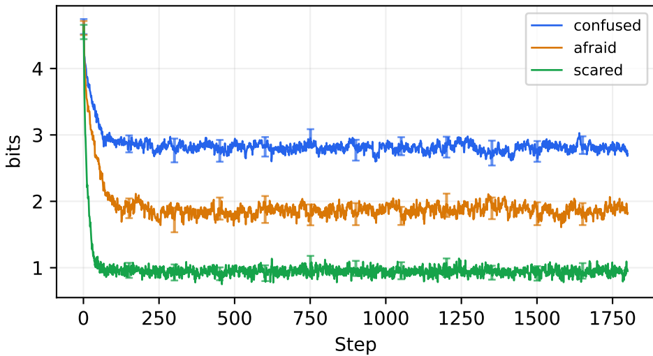
large_filter_walls: entropy
