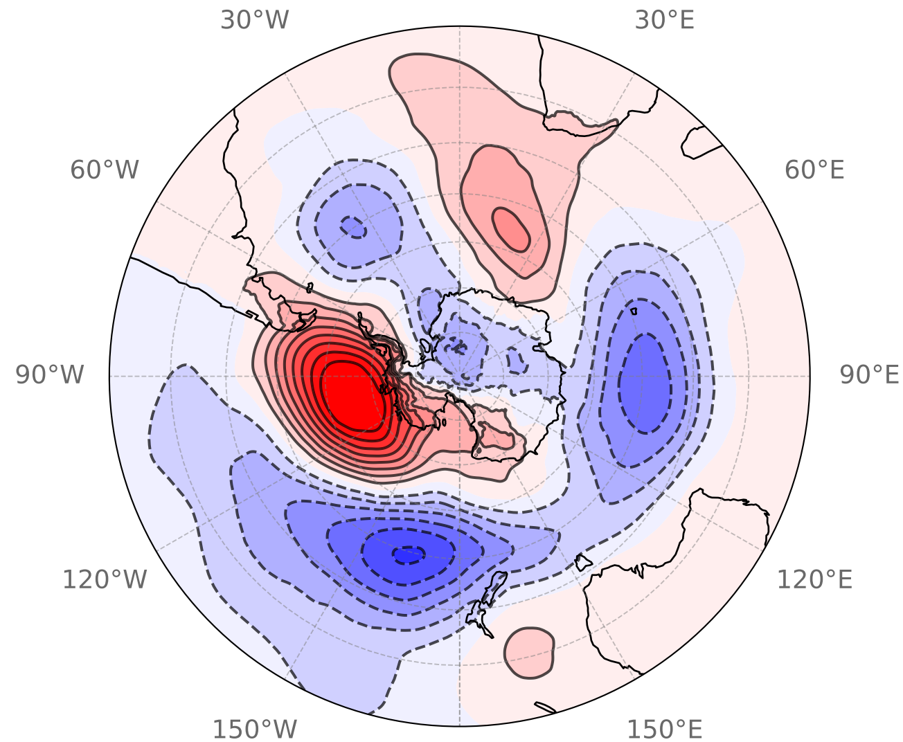
(b) Cluster 2 (SAM+) – Most positive PC1 (n=199)
