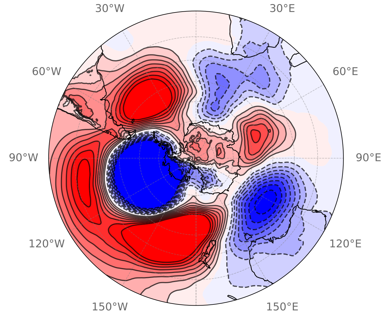
(c) Cluster 3 (SAM–) – Most negative PC1 (n=79)
