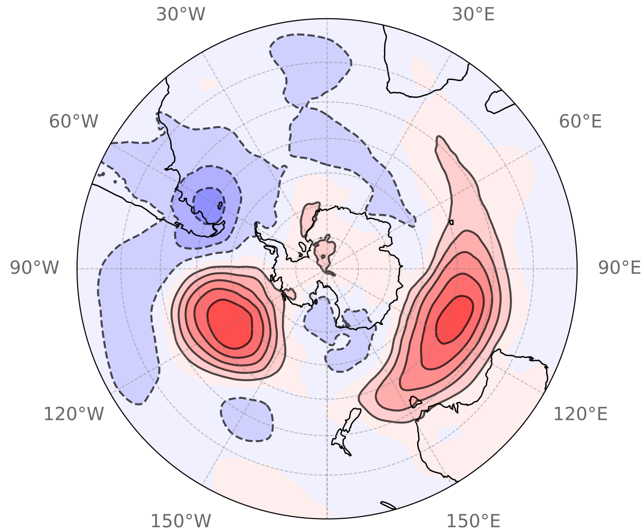
(a) Cluster 1 (Low-amplitude SAM–) – Near-zero PC1 (n=238)
