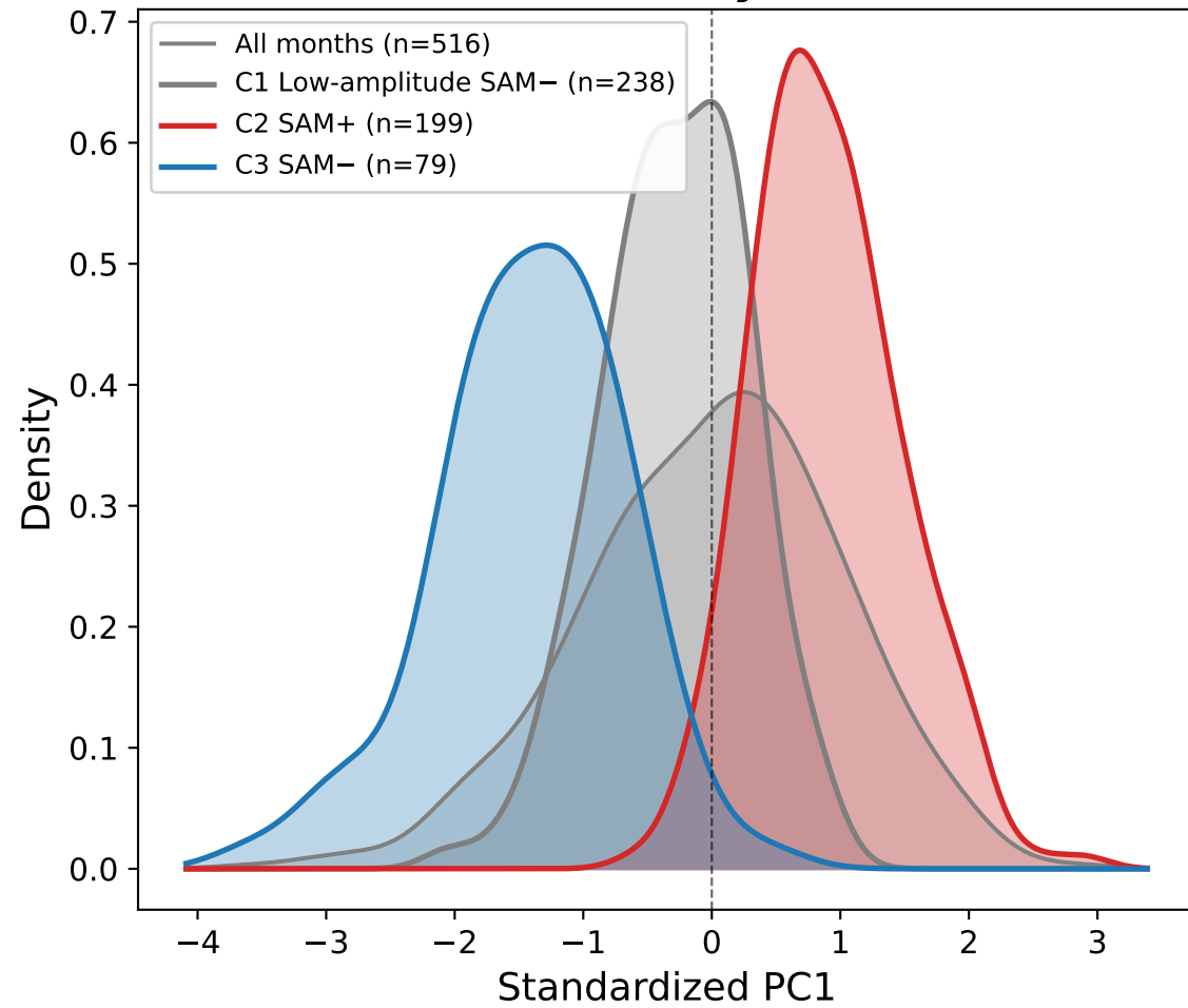
(a) Kernel density estimates
