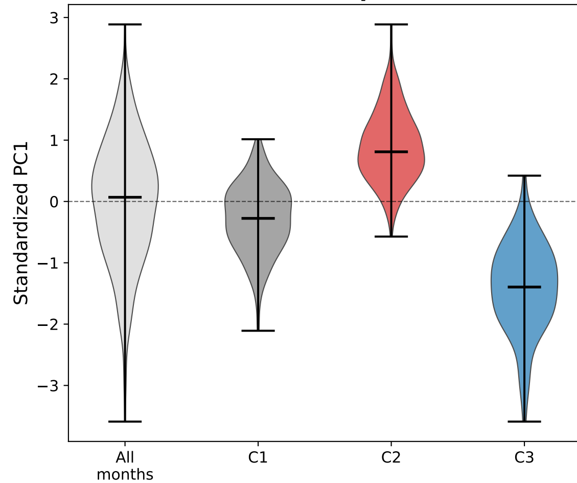
(c) Violin plot
