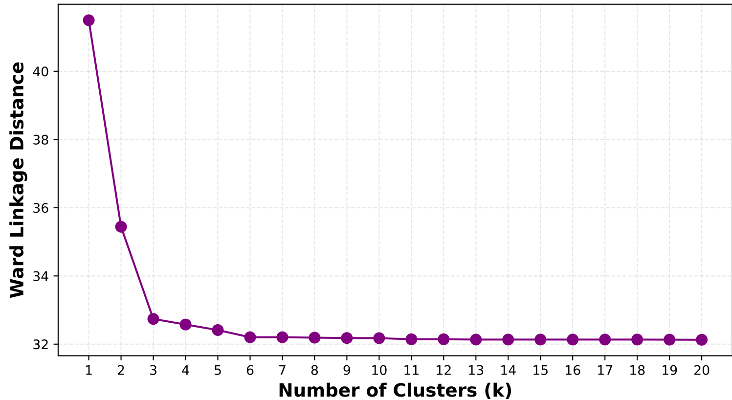
Elbow Plot for Principal Component Hierarchical Clustering (first 516 PC modes)
