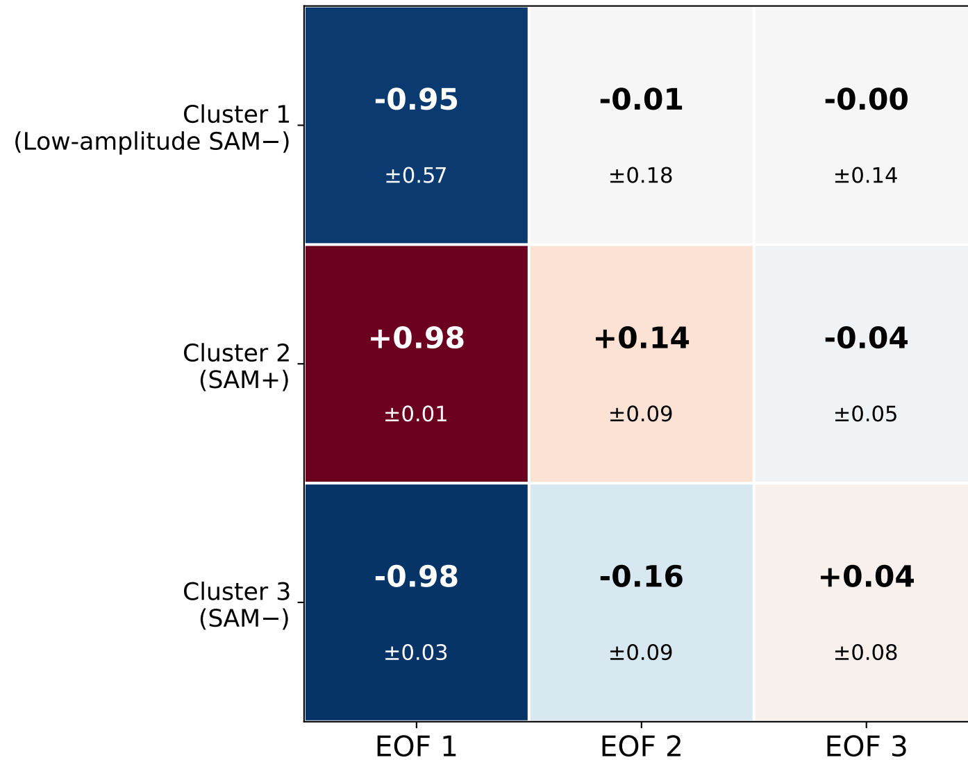
(a) Spatial Correlation Ensemble-mean composites vs EOF modes
