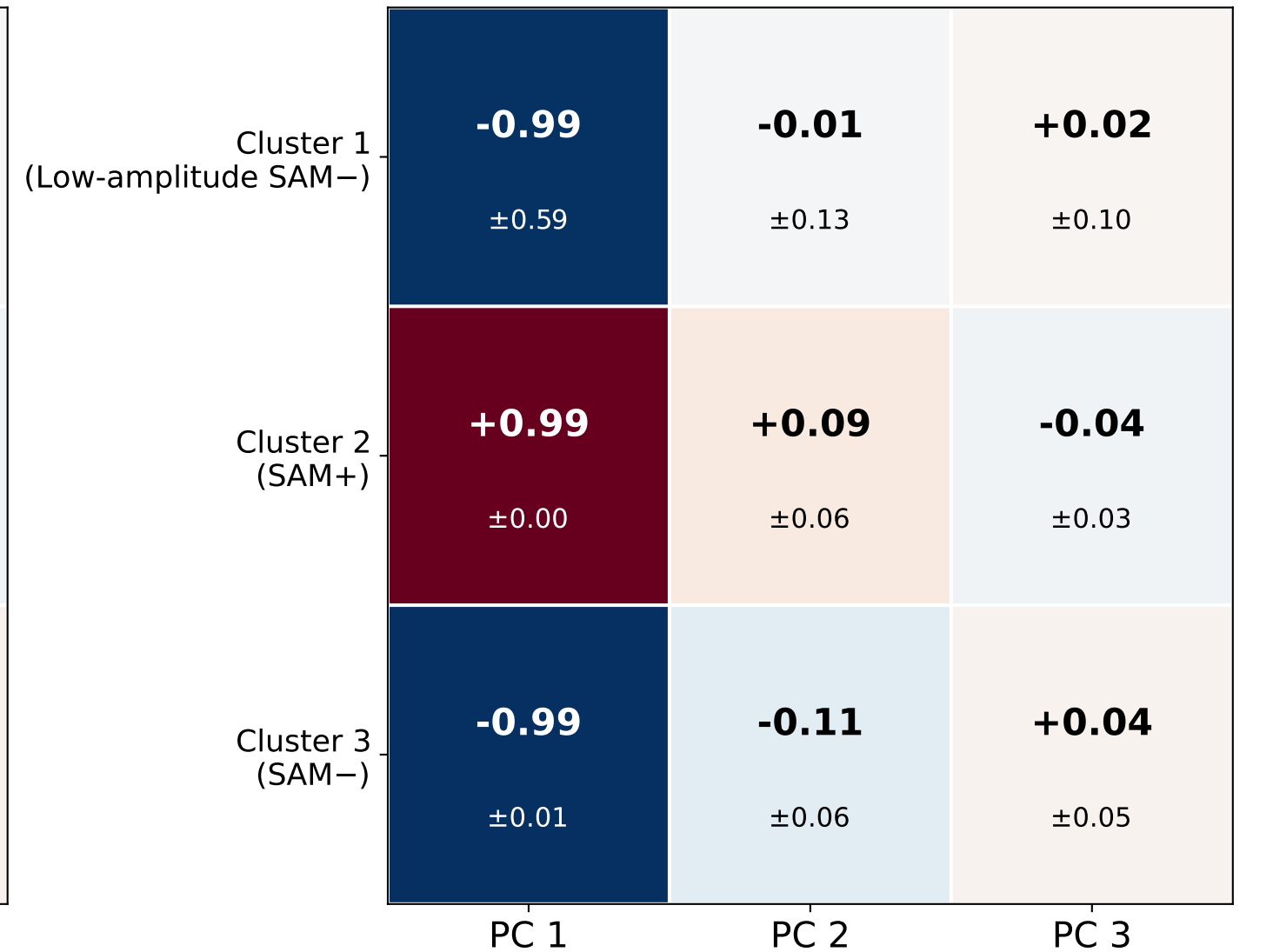
(b) Temporal Correlation Direct cluster projections vs PCs
