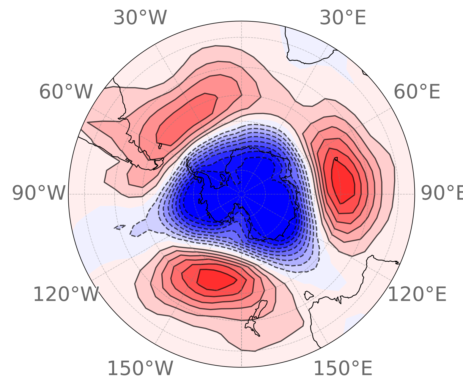
(e) MAM Cluster 4 10 events (7.8%)
