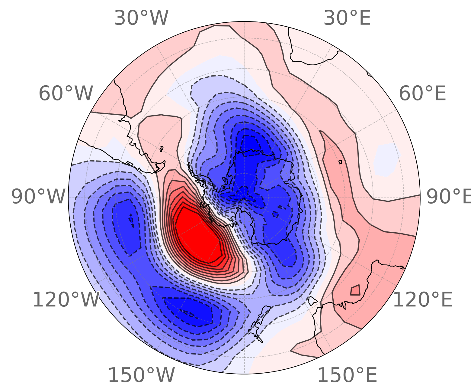
(c) MAM Cluster 2 31 events (24.0%)
