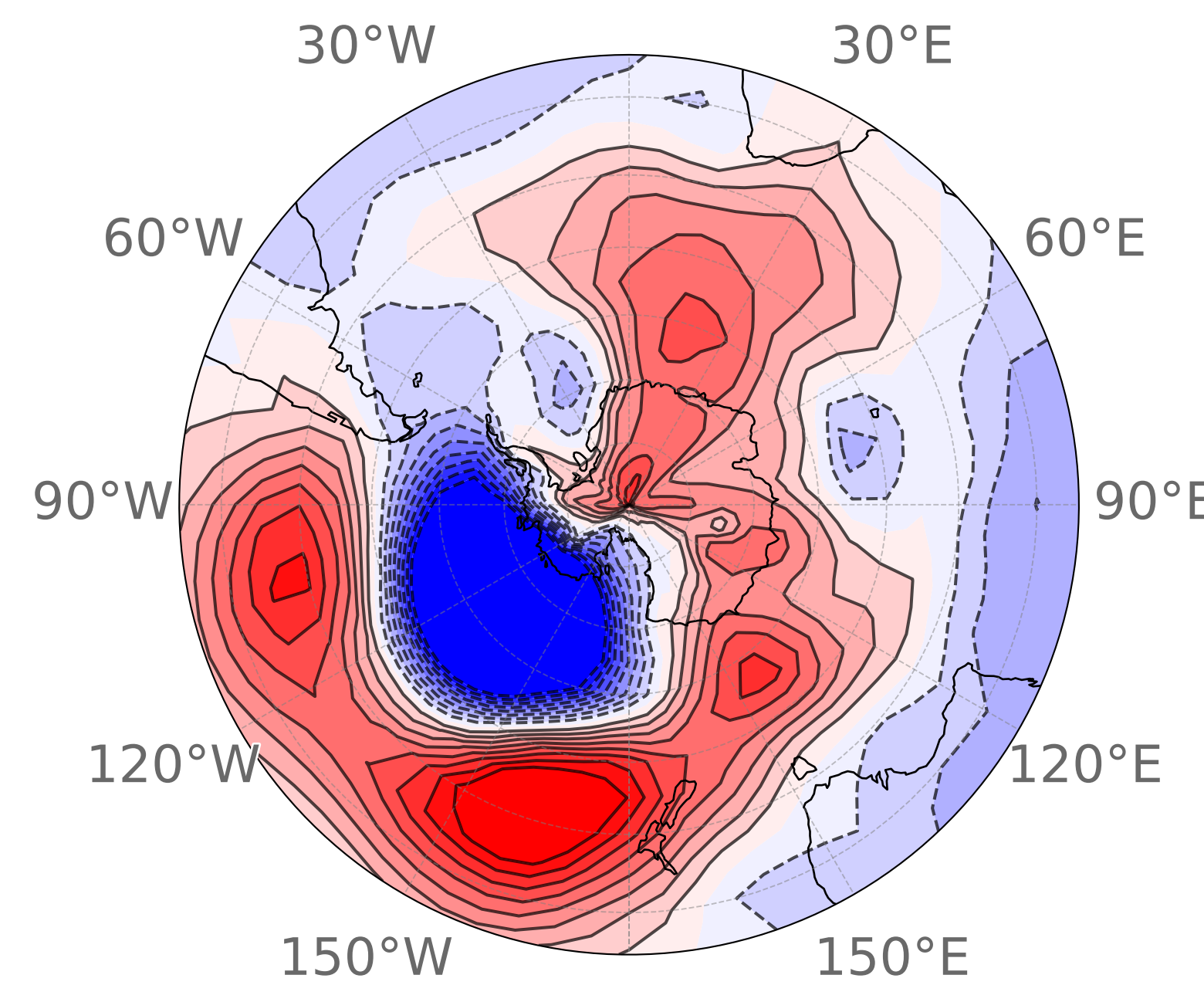
(b) MAM Cluster 1 62 events (48.1%)
