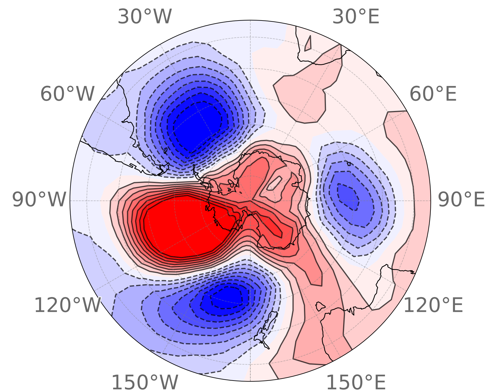
(b) SON Cluster 1 64 events (49.6%)
