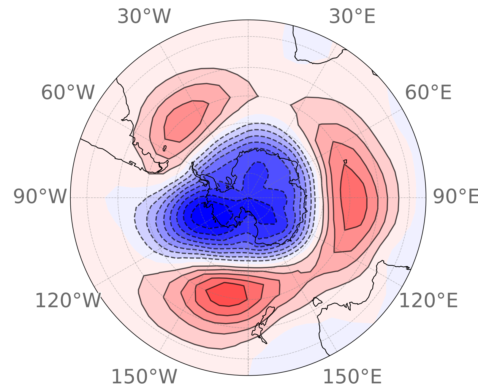
(c) SON Cluster 2 45 events (34.9%)
