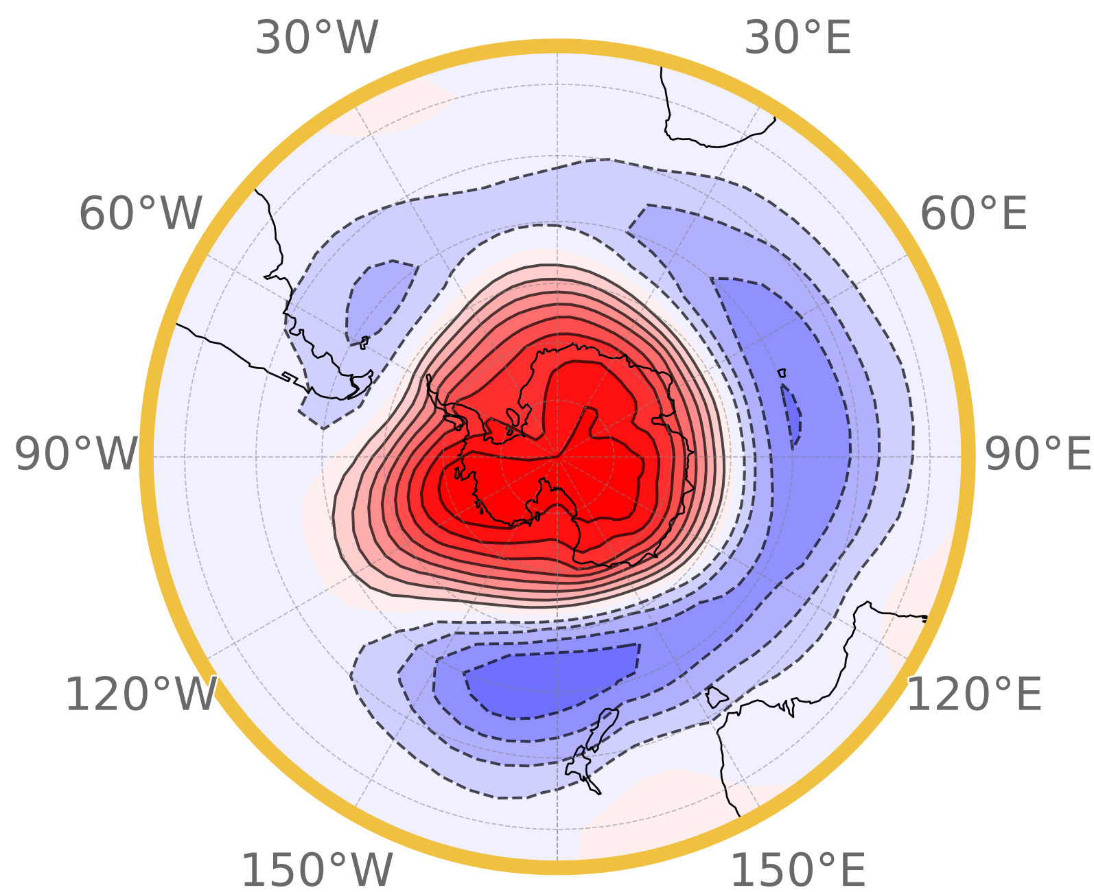
(a) SON EOF 1 reference
