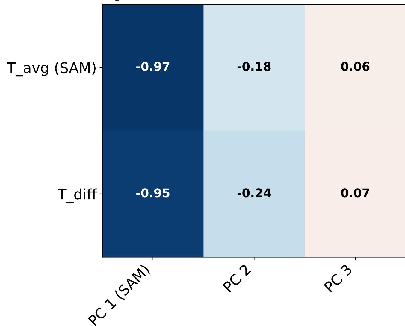
(b) Temporal Correlation Temporal Reconstruction vs PCs
