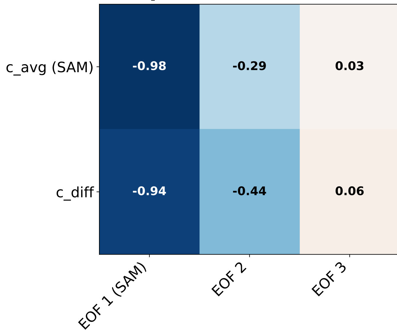
(a) Spatial Correlation Basis patterns vs EOF modes
