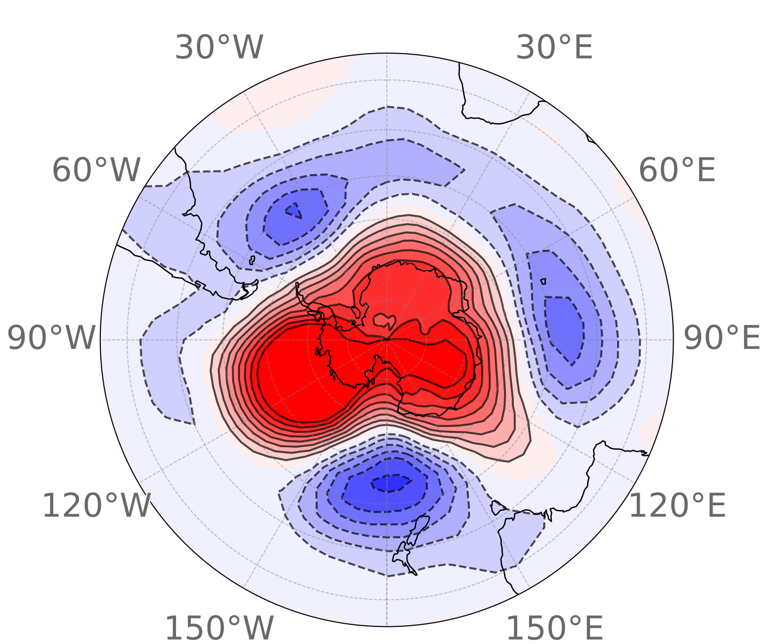
(j) MAM Cluster 4 5 events (3.9%)
