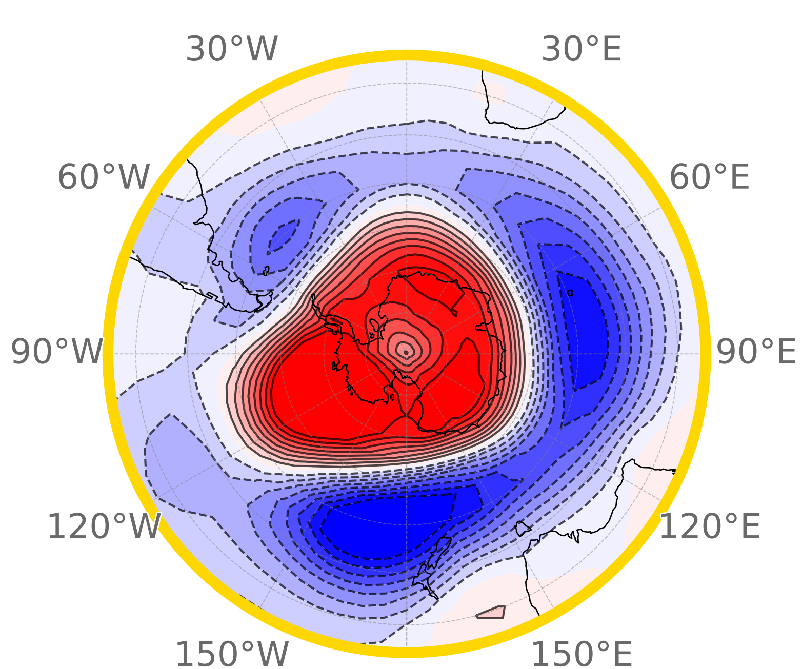
(o) SON EOF 1 reference
