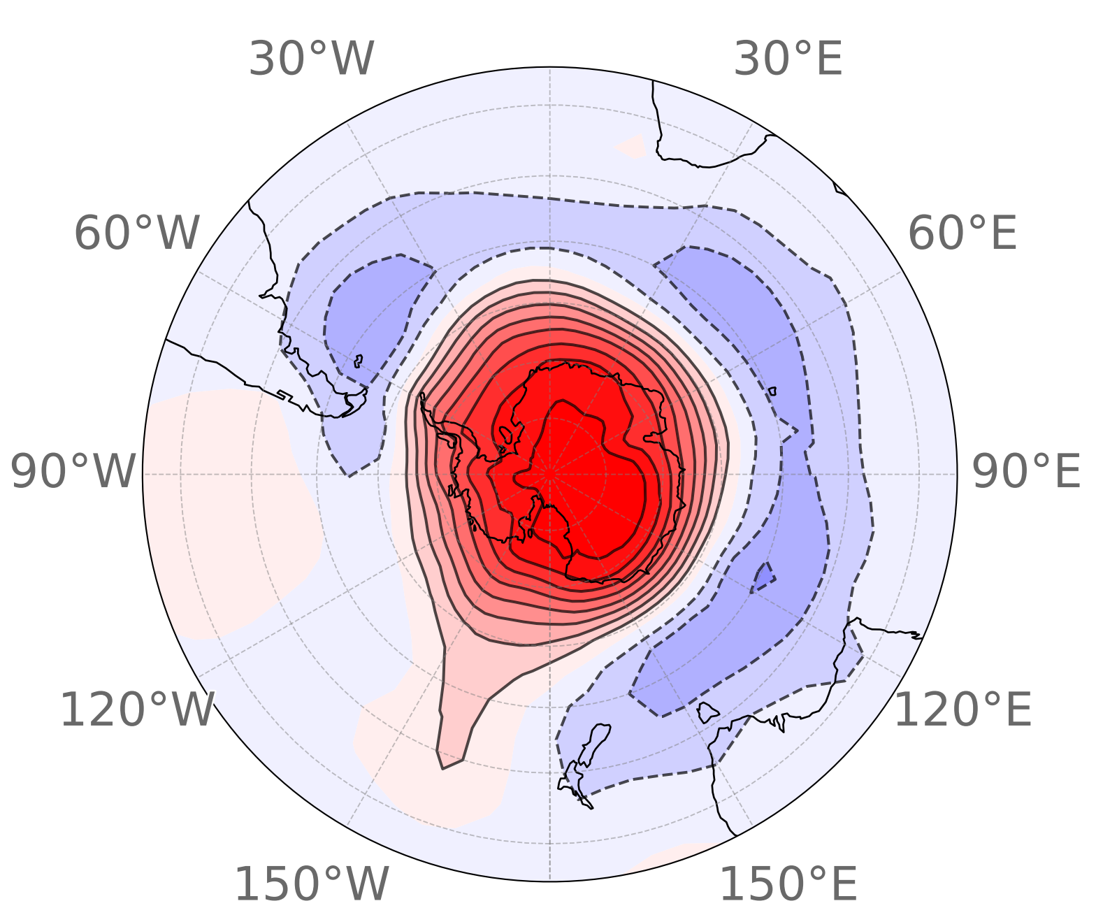
(e) DJF Cluster 4 12 events (9.3%)
