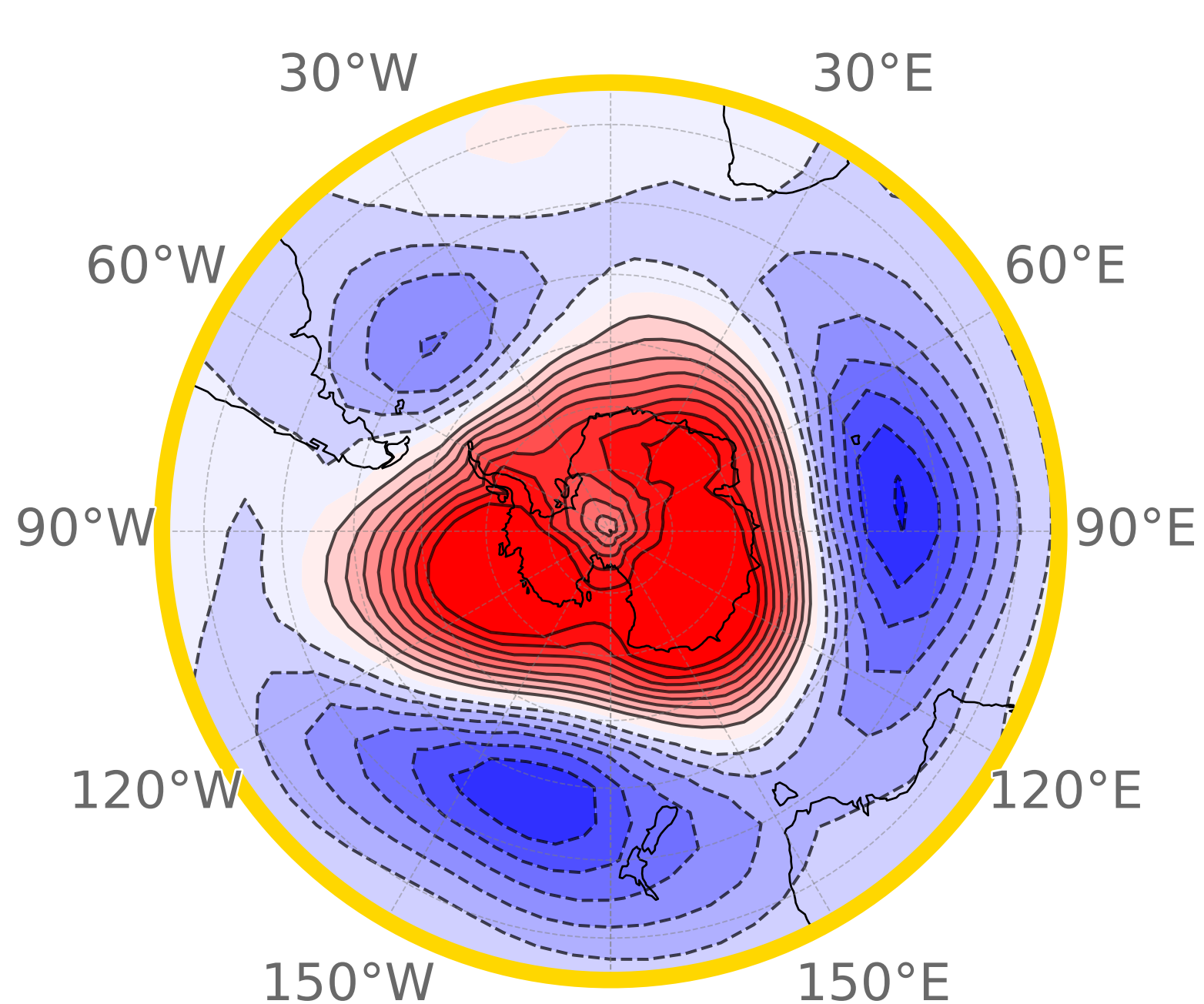
(k) JJA EOF 1 reference
