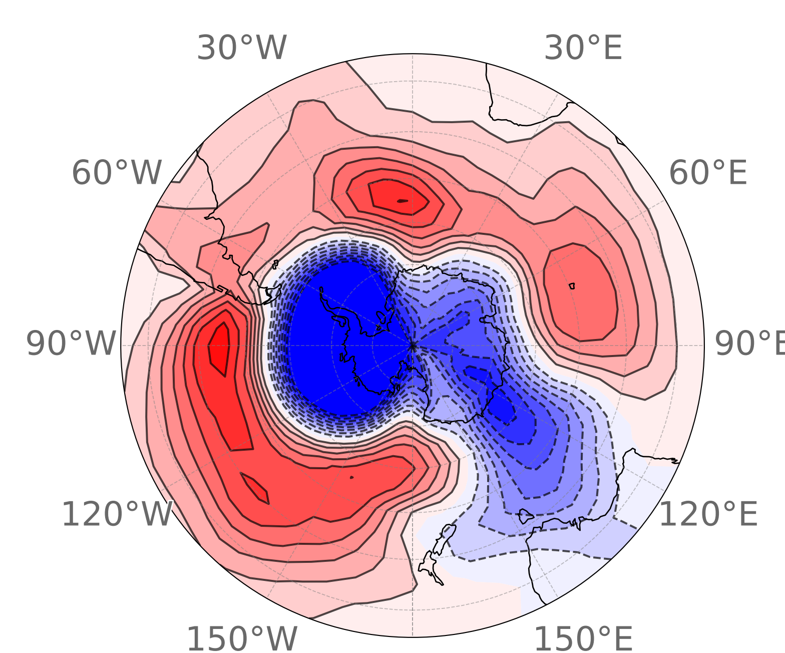
(l) JJA Cluster 1 61 events (47.3%)
