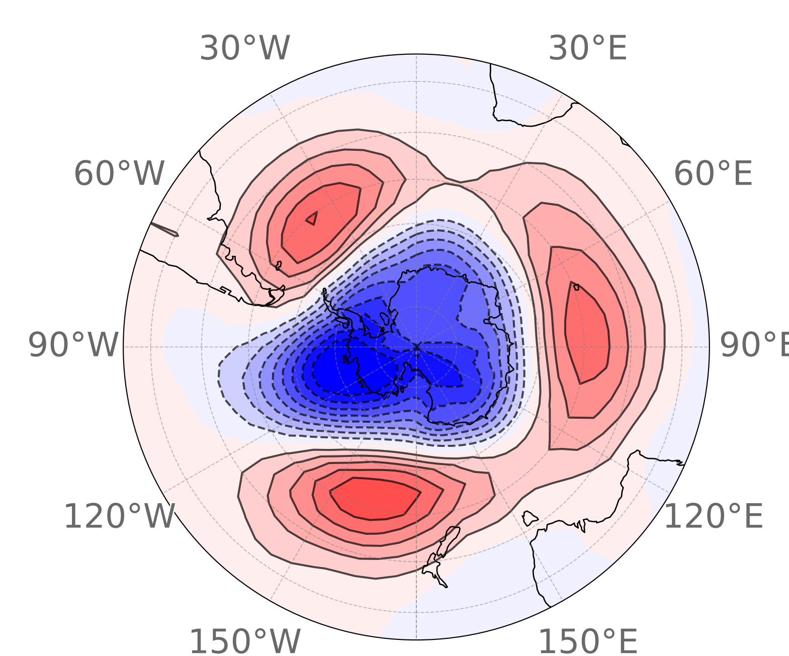
(q) SON Cluster 2 26 events (20.2%)
