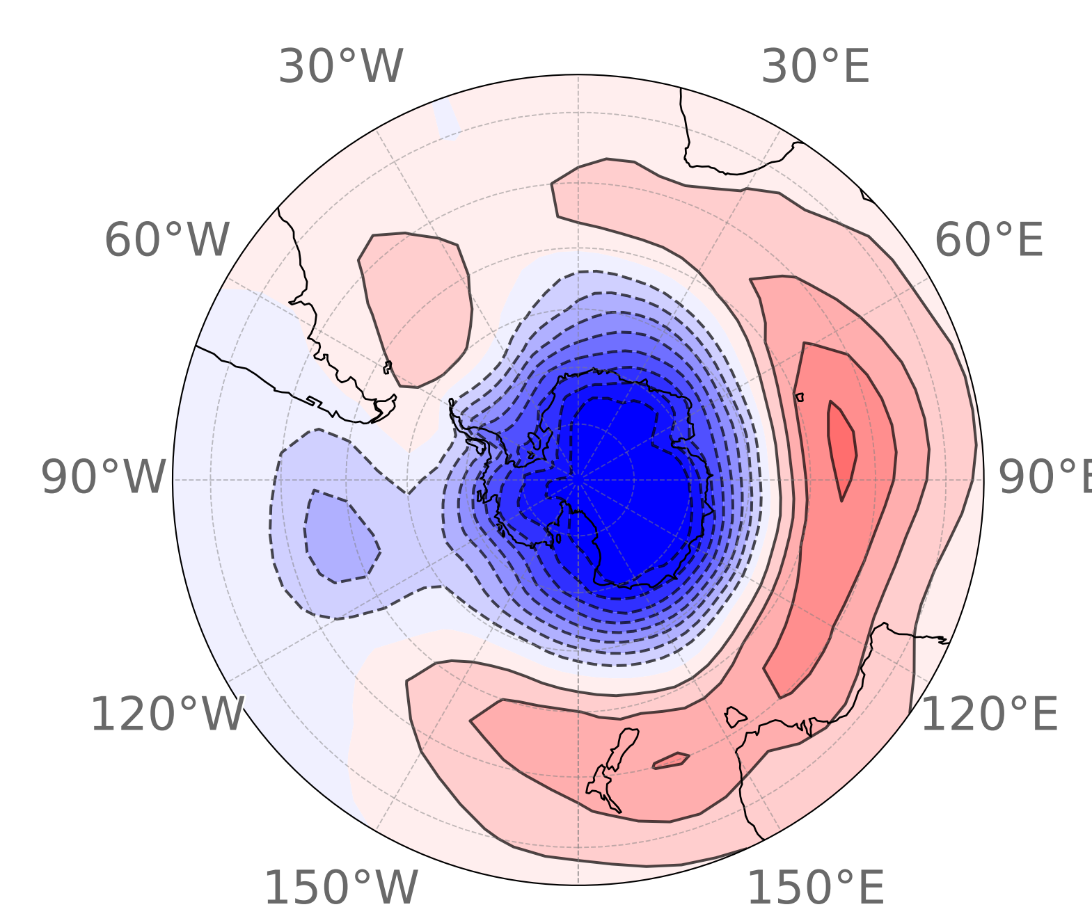
(n) JJA Cluster 3 24 events (18.6%)
