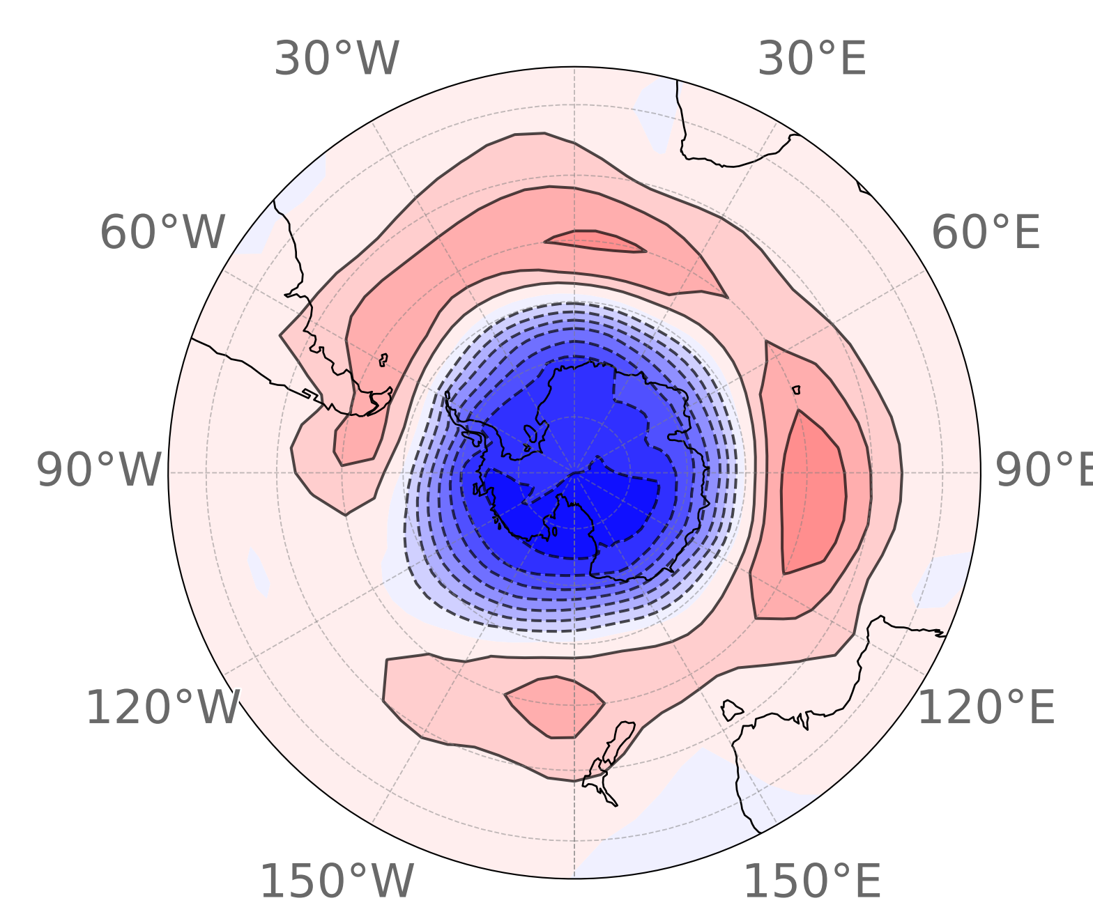
(b) DJF Cluster 1 49 events (38.0%)
