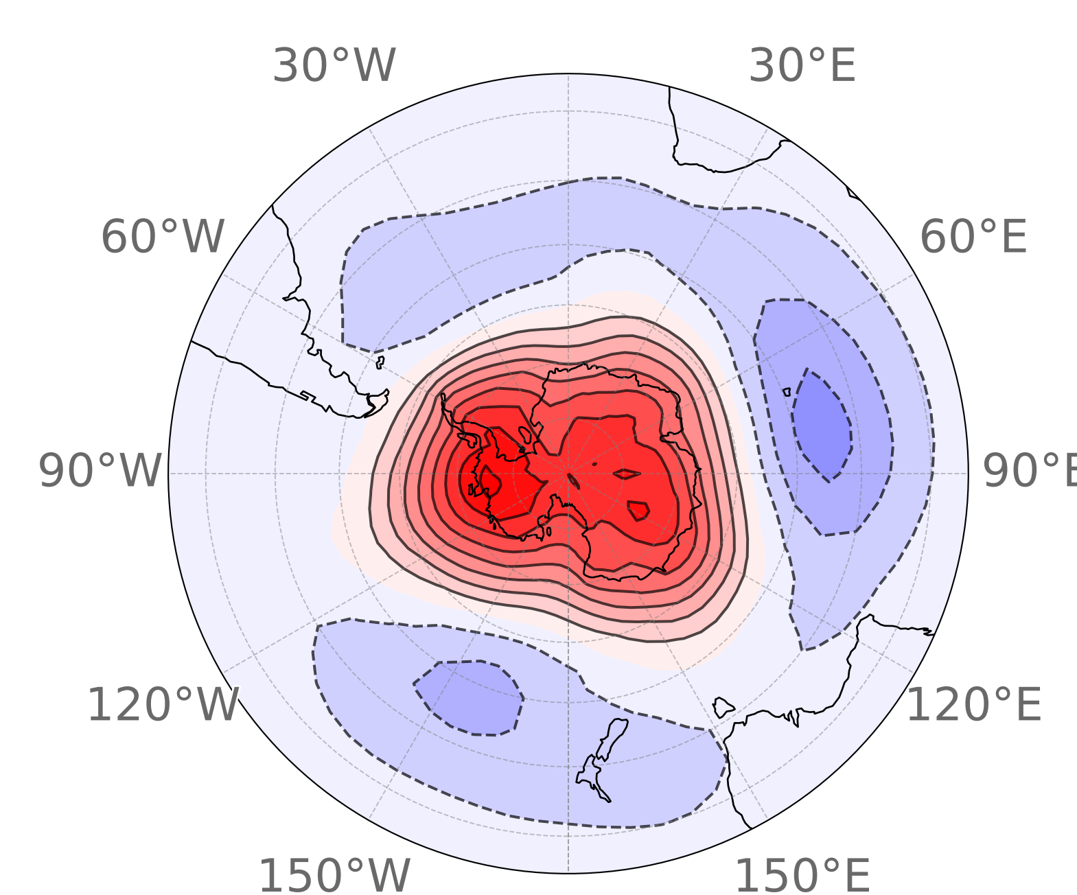
(m) JJA Cluster 2 44 events (34.1%)
