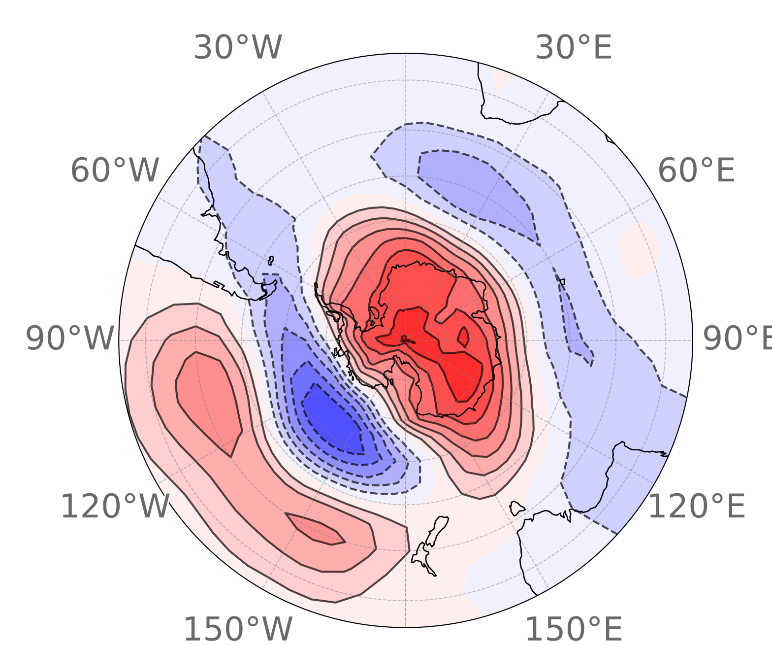
(g) MAM Cluster 1 67 events (51.9%)
