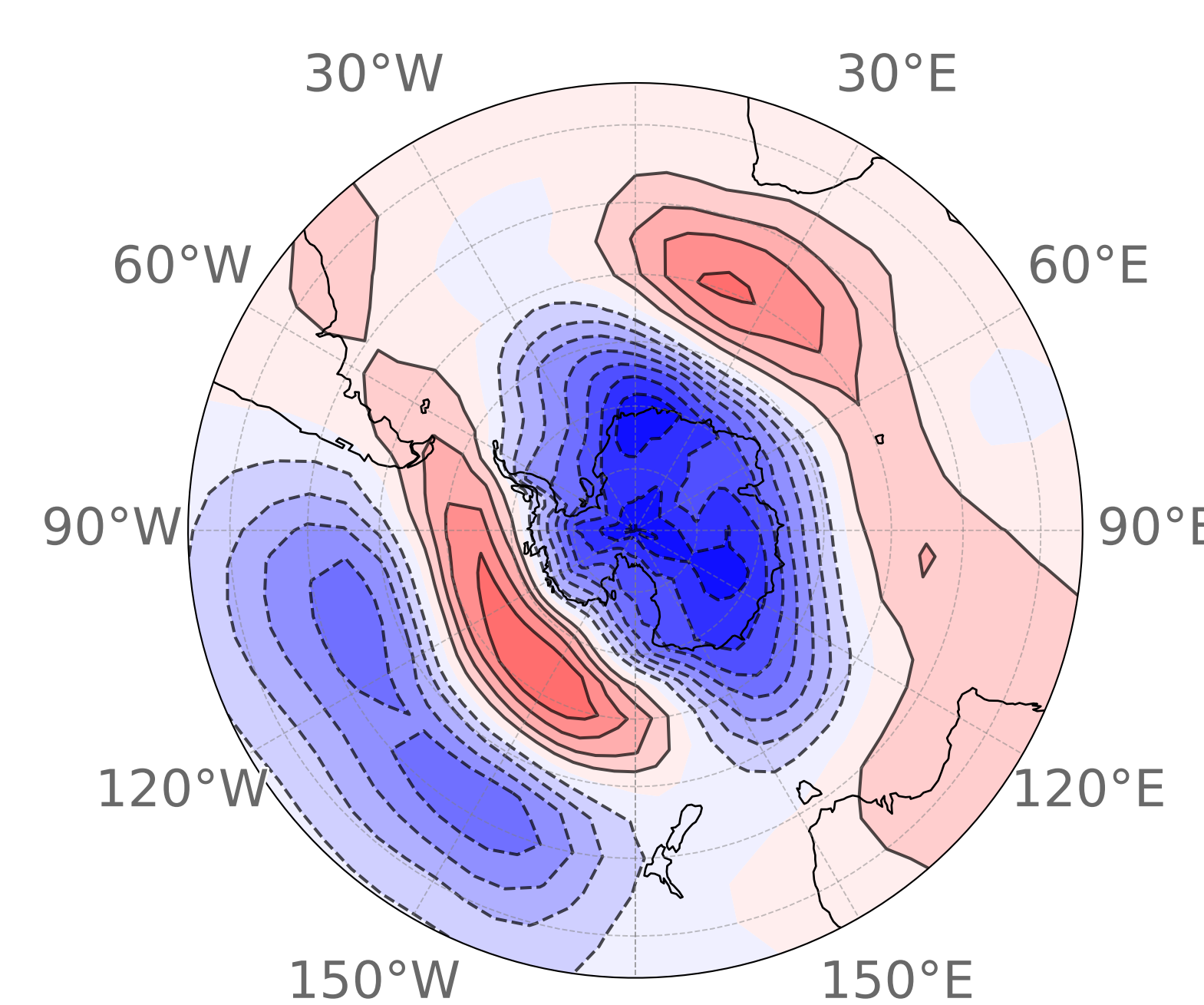
(h) MAM Cluster 2 50 events (38.8%)
