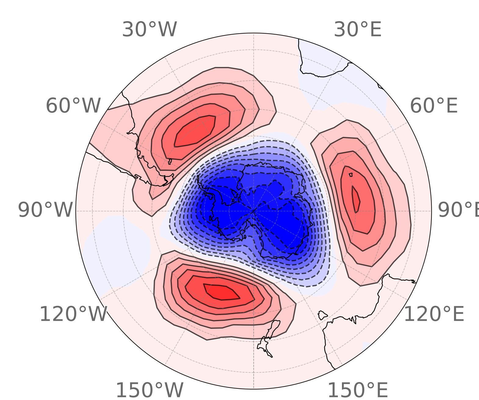
(i) MAM Cluster 3 7 events (5.4%)
