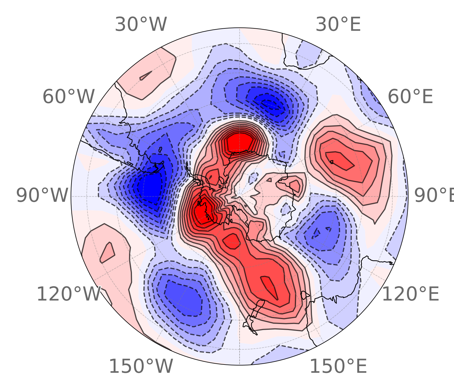
(c) DJF Cluster 2 48 events (37.2%)
