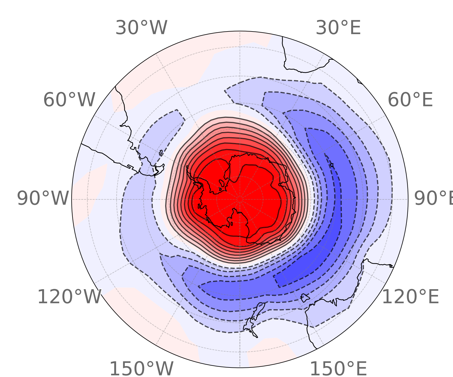
(r) SON Cluster 3 19 events (14.7%)
