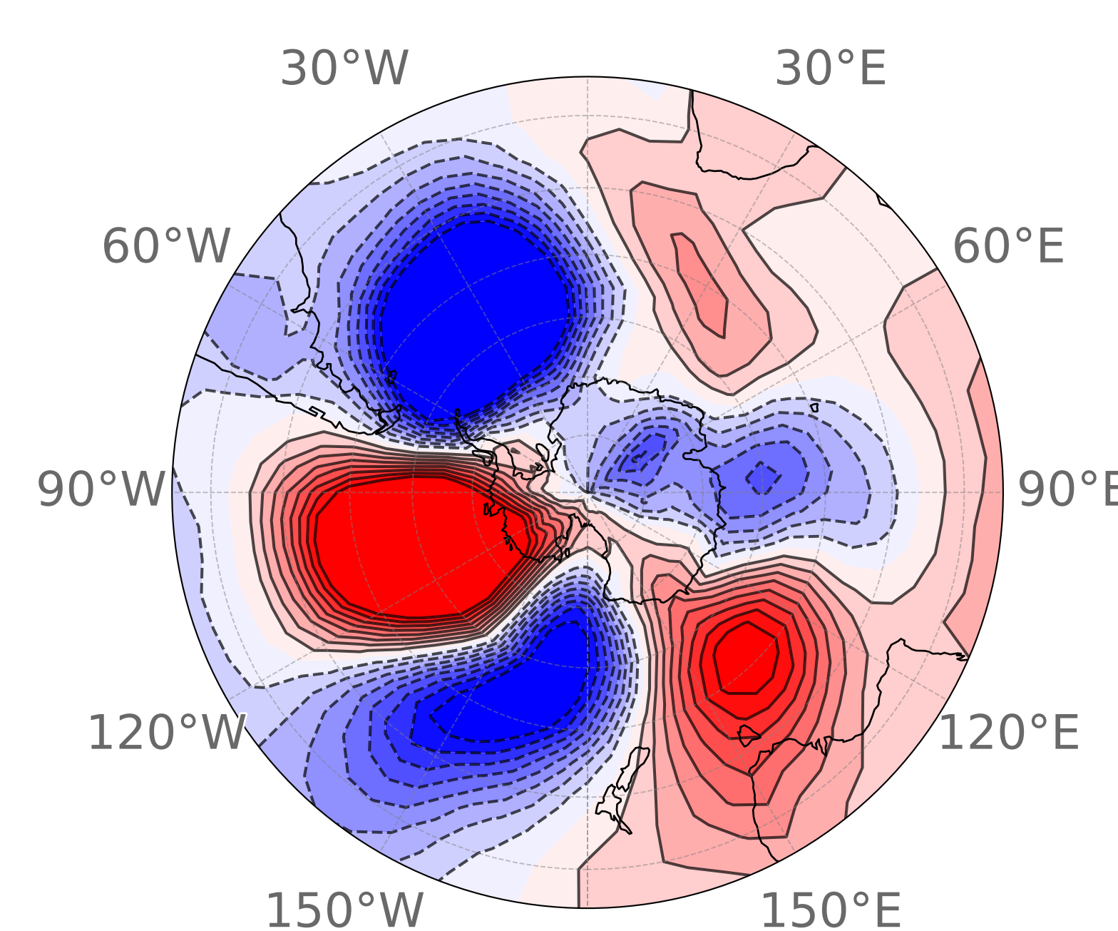
(p) SON Cluster 1 84 events (65.1%)
