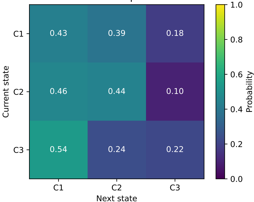
Cluster transition probabilities
