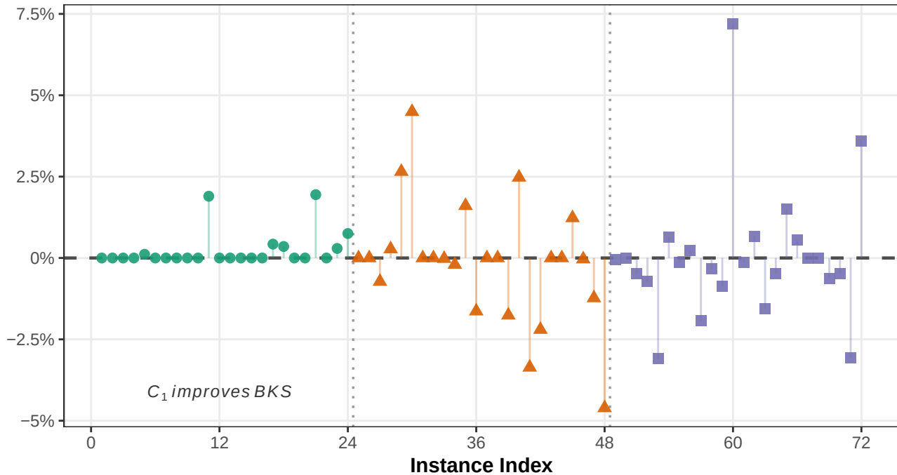
Relative Percentage Deviation to BKS (RPD BKS )
