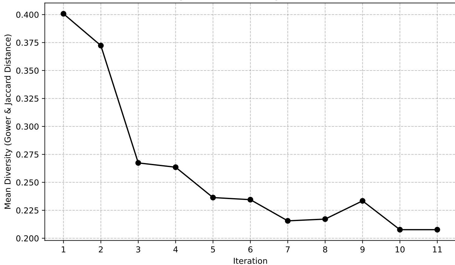
Convergence of Elite Configurations (iRace)
