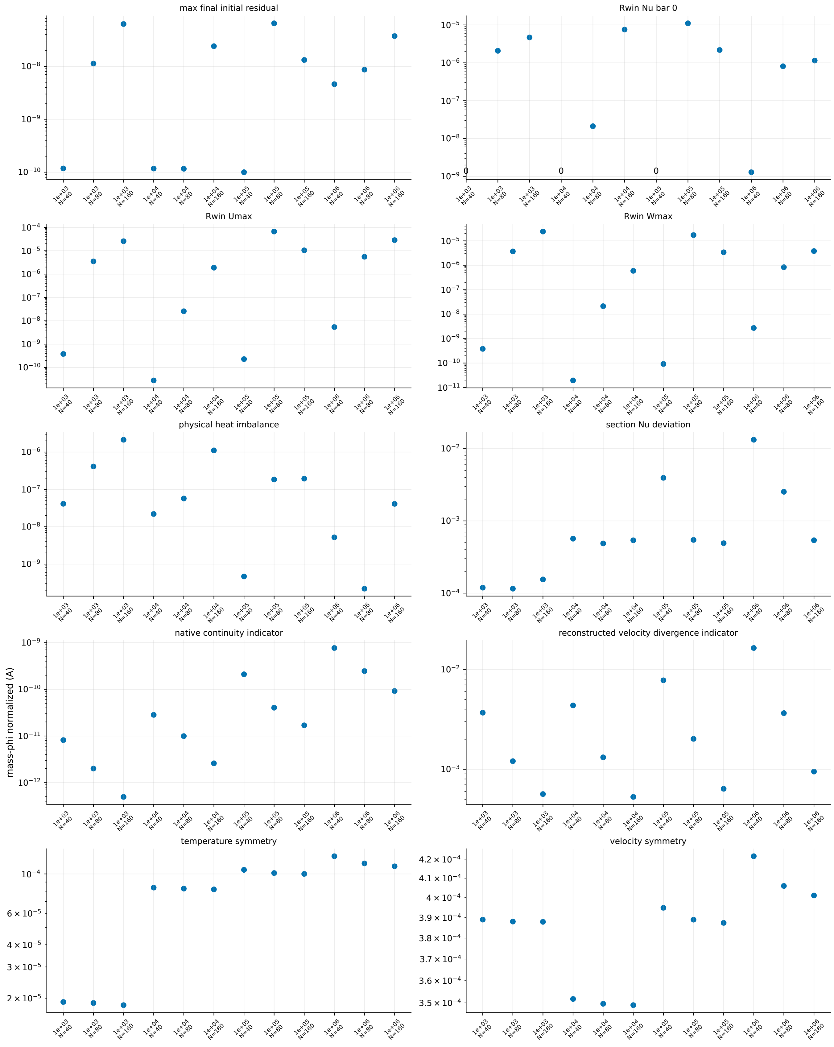
Route A: convergence and conservation diagnostics Native phi indicators have different operators/units between routes; hollow markers = diagnostic-only
