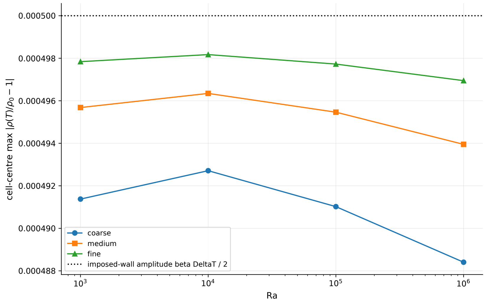
Route A: temperature-dependent EOS; \psi = 0
