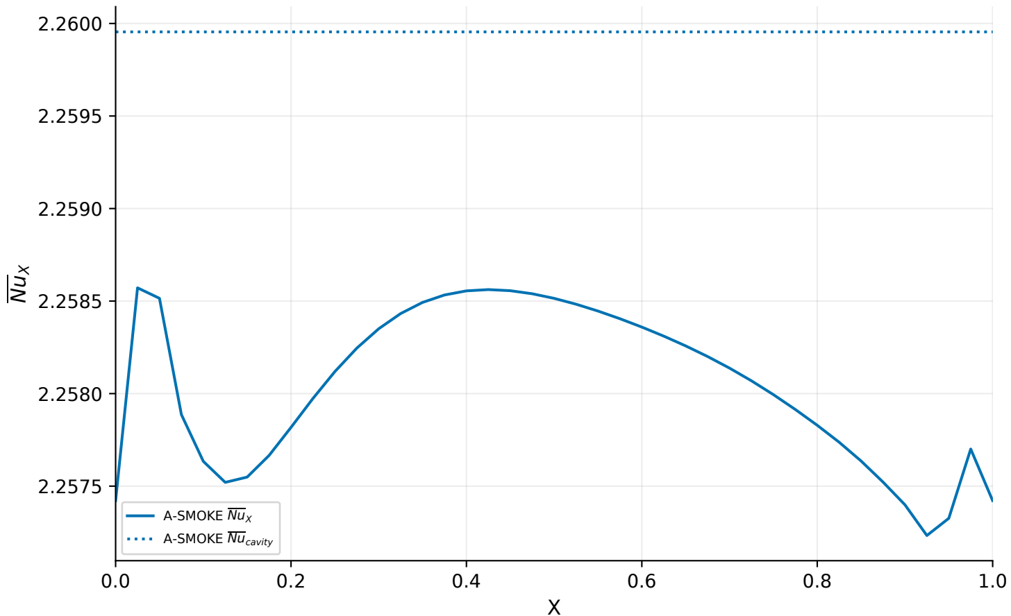
A-SMOKE Route A | Ra=10000 | 40x40x1 | auxiliary (outside formal matrix) A: interpolated cell U
