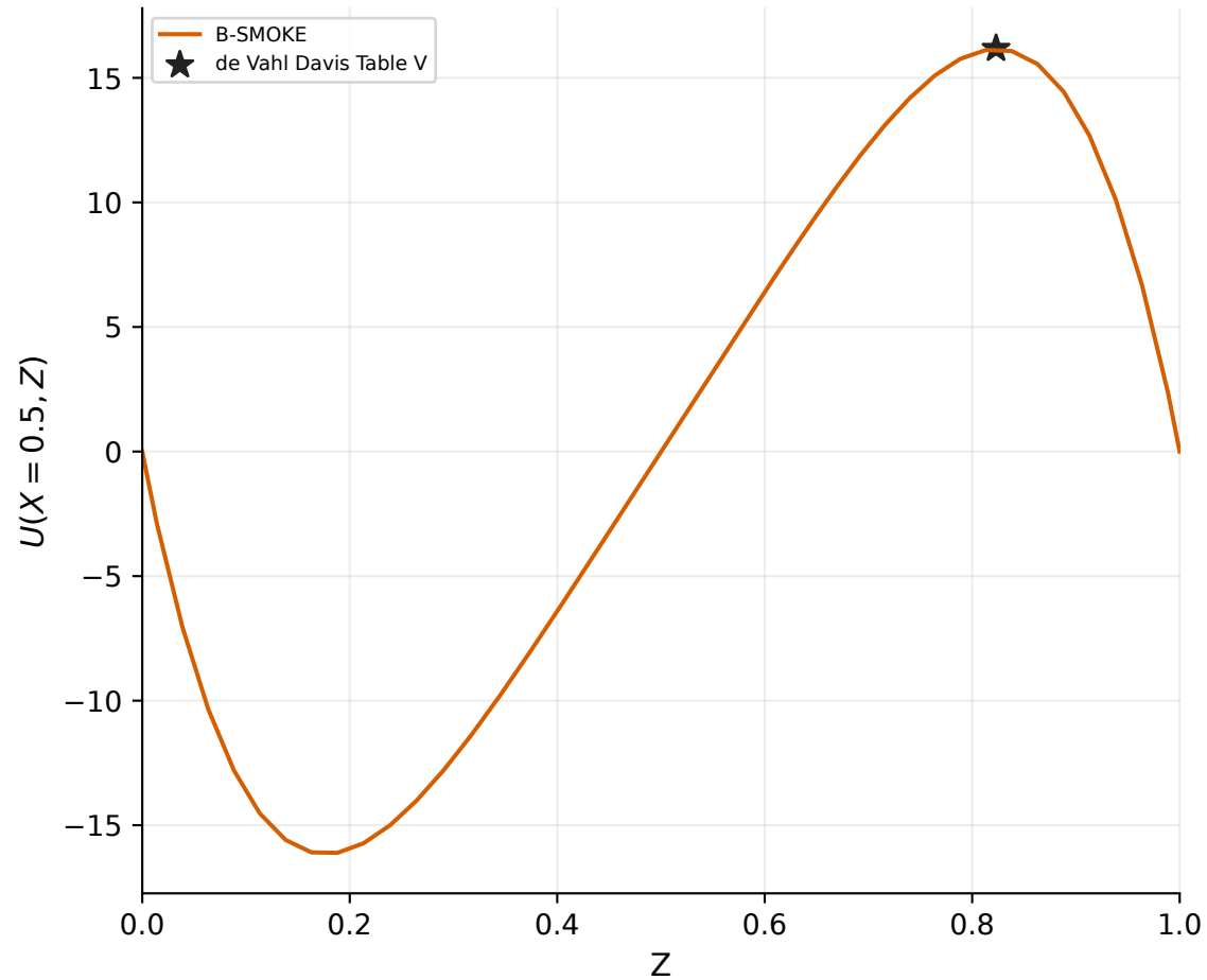
B-SMOKE Route B | Ra=10000 | 40x40x1 | auxiliary (outside formal matrix)
