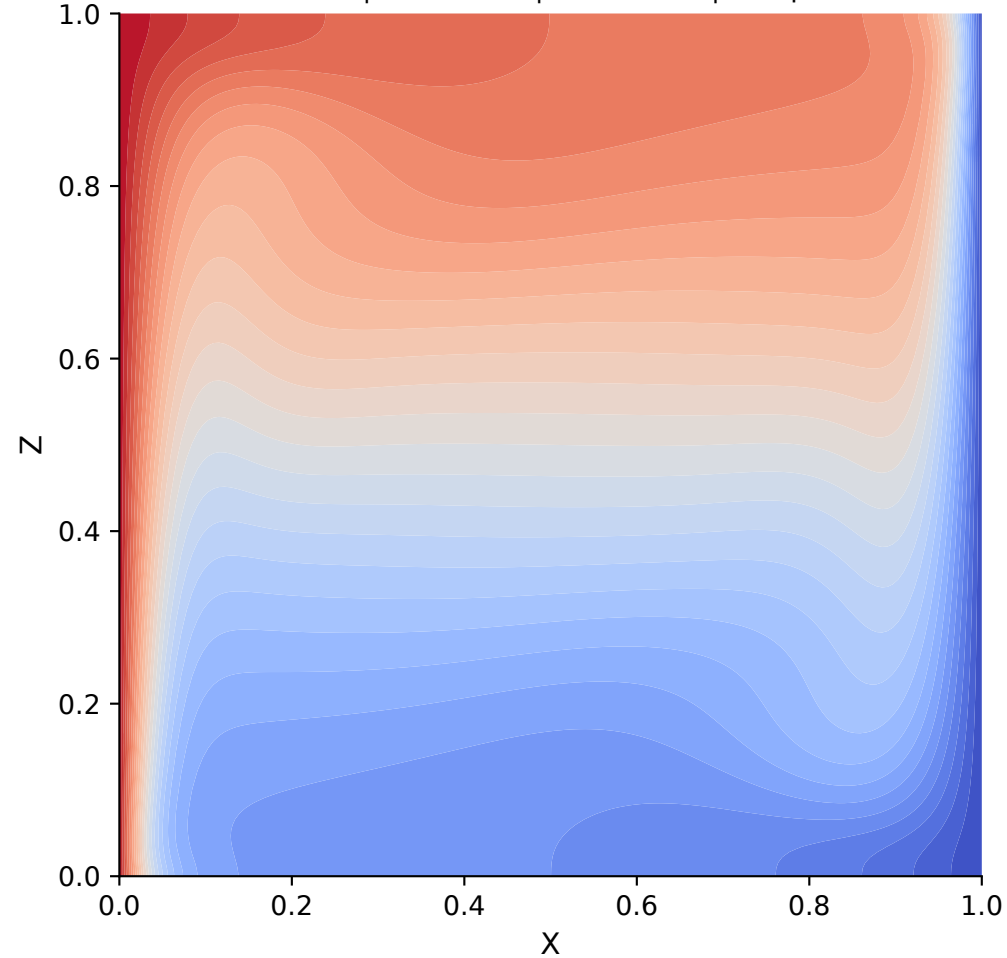
A-Ra1e6-fine Route A | Ra=1e+06 | 160x160x1 | accepted
