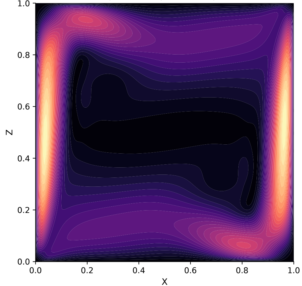
A-Ra1e6-fine Route A | Ra=1e+06 | 160x160x1 | accepted
