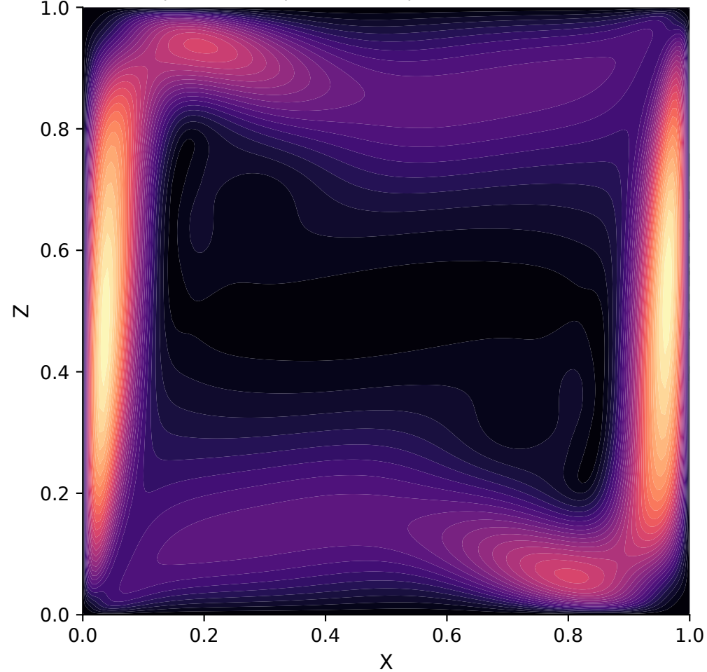
B-Ra1e6-fine Route B | Ra=1e+06 | 160x160x1 | diagnostic-only / unaccepted
